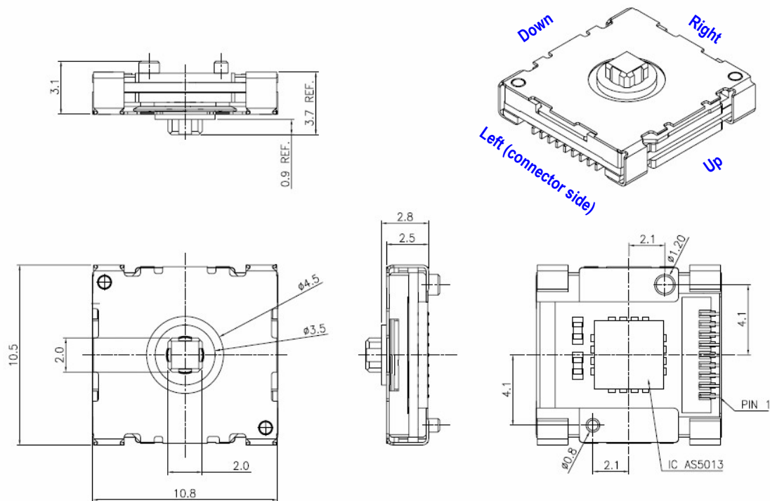
Figure 18. N35P112 Dimensions (mm \pm 0.15 )
