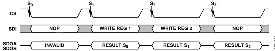
Figure 41. Register Write
