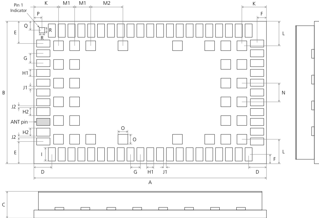
Figure 14: SARA-U2 series dimensions (bottom and sides views)
