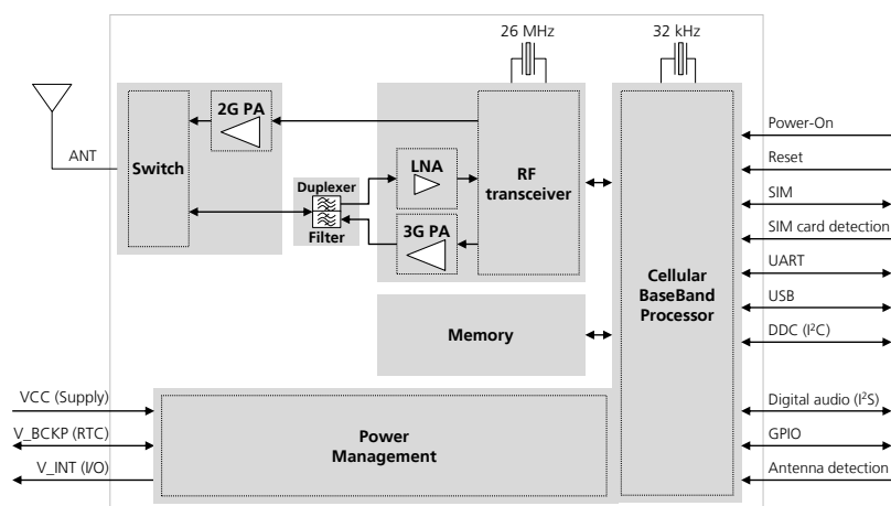
Figure 2: SARA-U260 and SARA-U270 block diagram
