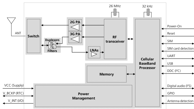
Figure 1: SARA-U201 block diagram
