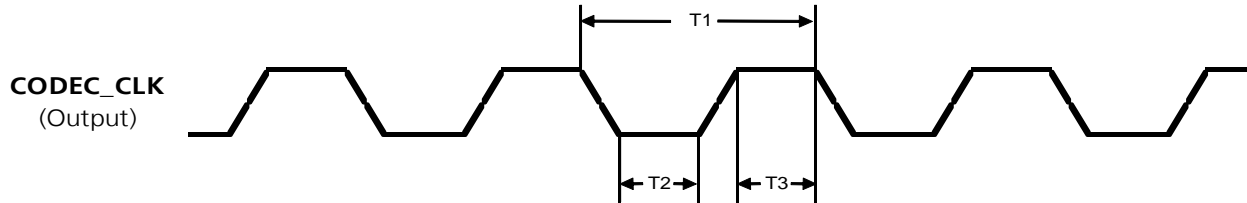
Figure 13: AC characteristics of CODEC_CLK digital clock output
