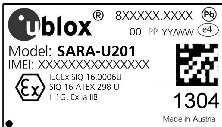
Figure 19: SARA-U201 ATEX modules label
