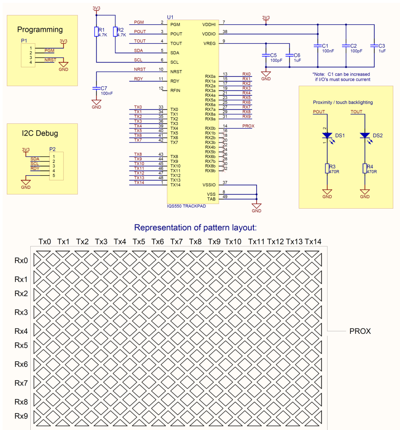
Figure 6.5 IQS550 Application Circuit
