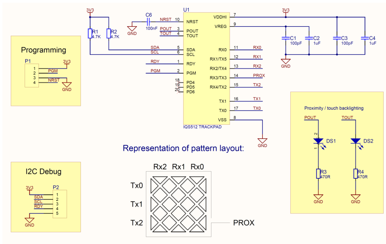
Figure 6.8 IQS512 Application Circuit
