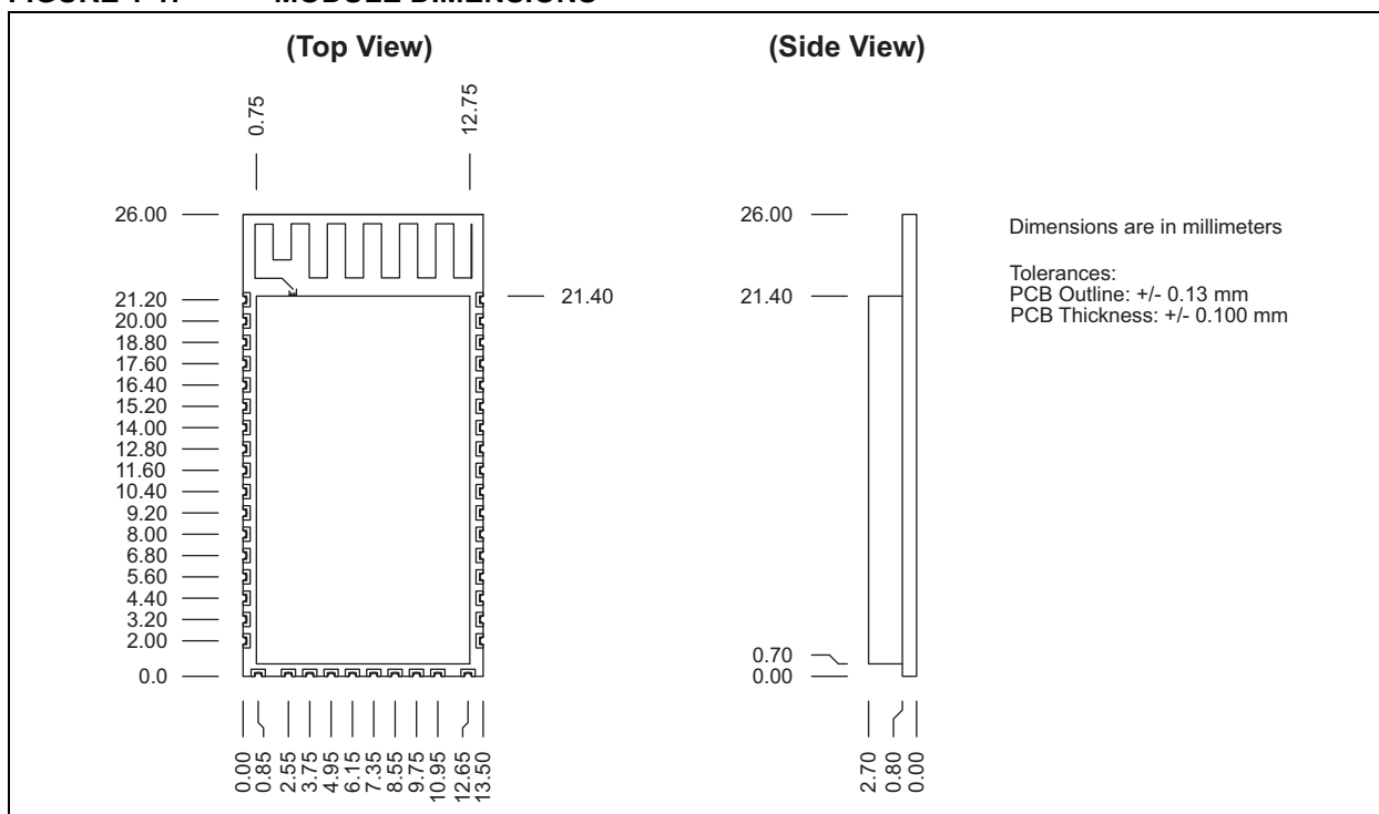
FIGURE 1-1: MODULE DIMENSIONS
