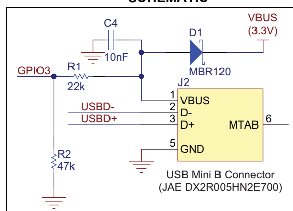
FIGURE 2-4: USB DFU PORT & GPIO3 SCHEMATIC
