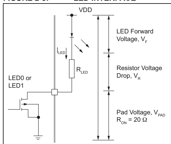
FIGURE 2-3: LED INTERFACE
