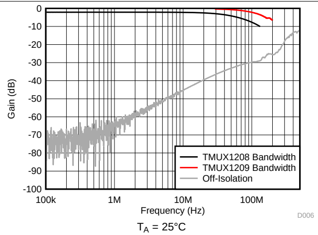
Figure 6. Frequency Response
