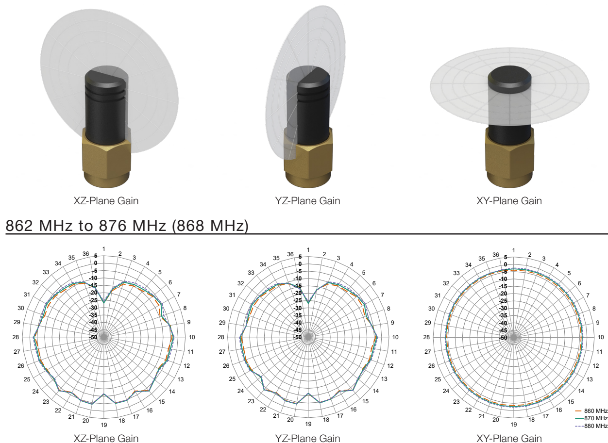
Figure 16. Radiation Patterns for ANT-868-NUB-ccc Antenna in Free Space
