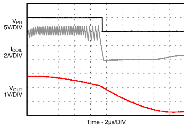
Figure 8-27. HICCUP Short Circuit Protection (Zoom In)
