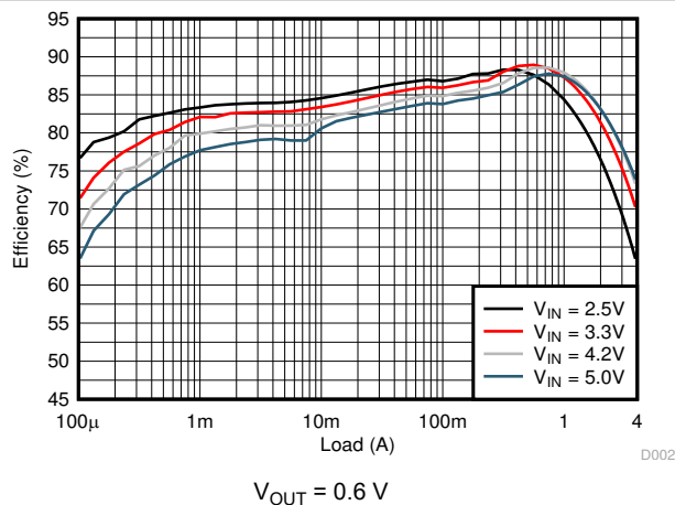
Figure 8-2. Efficiency
