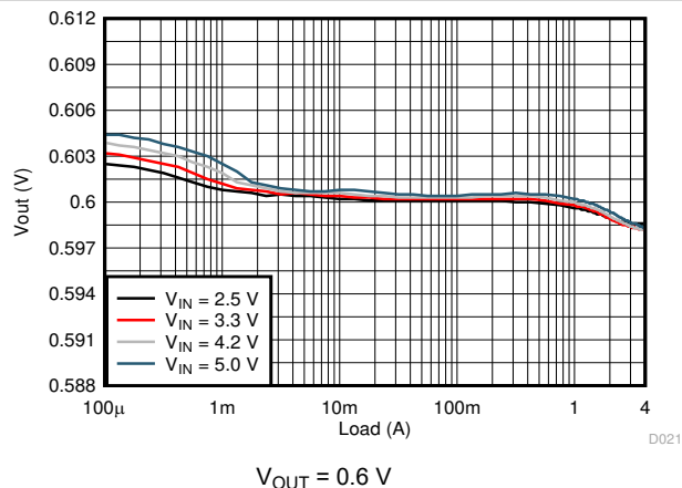
Figure 8-3. Load Regulation
