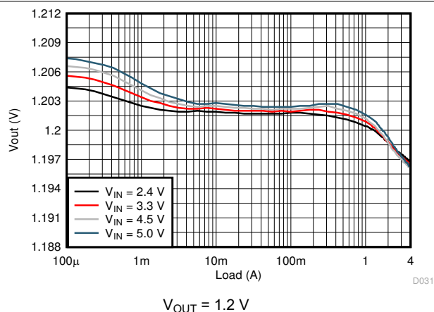
Figure 8-5. Load Regulation
