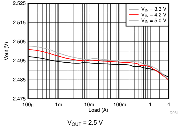
Figure 8-9. Load Regulation
