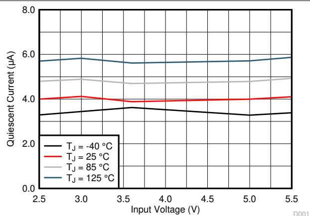
Figure 6-4. Quiescent Current
