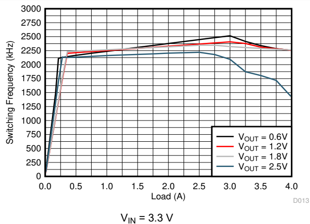
Figure 8-12. Switching Frequency
