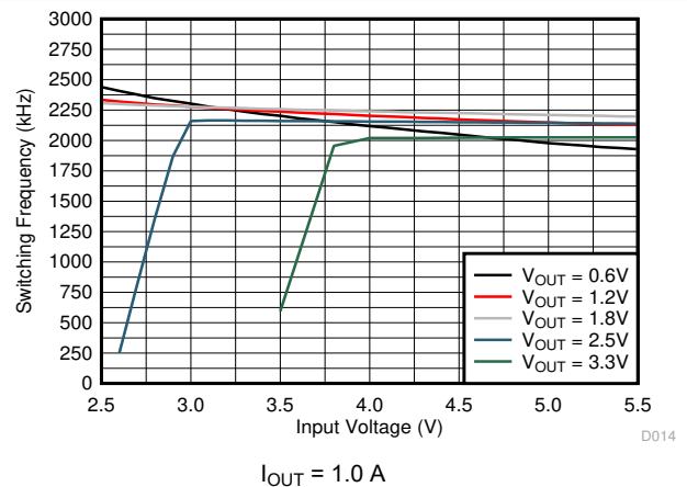
Figure 8-13. Switching Frequency
