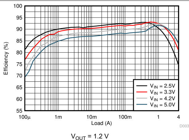
Figure 8-4. Efficiency
