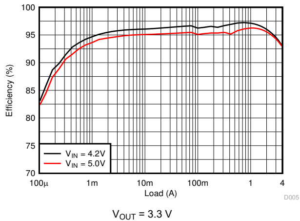
Figure 8-10. Efficiency
