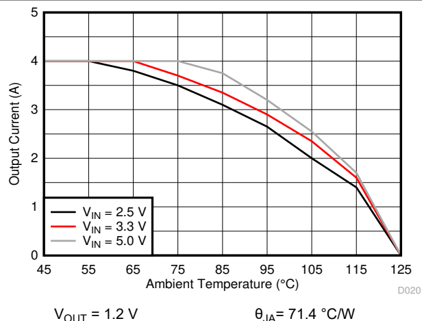
Figure 8-14. Thermal Derating
