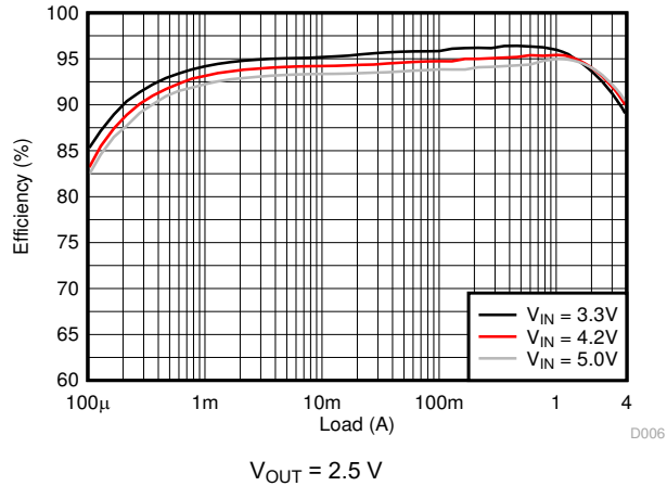
Figure 8-8. Efficiency
