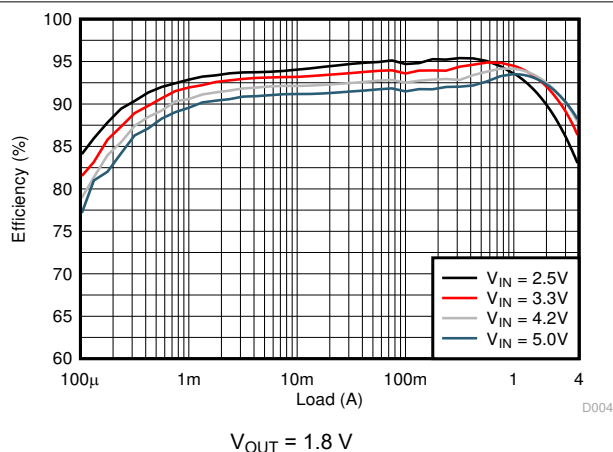
Figure 8-6. Efficiency
