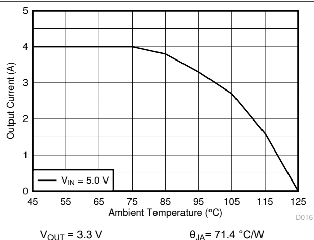
Figure 8-17. Thermal Derating
