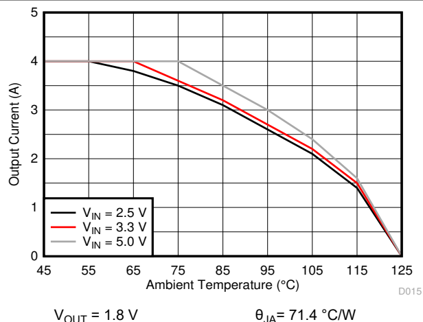
Figure 8-15. Thermal Derating
