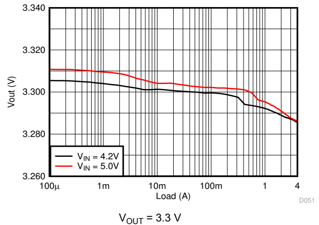
Figure 8-11. Load Regulation
