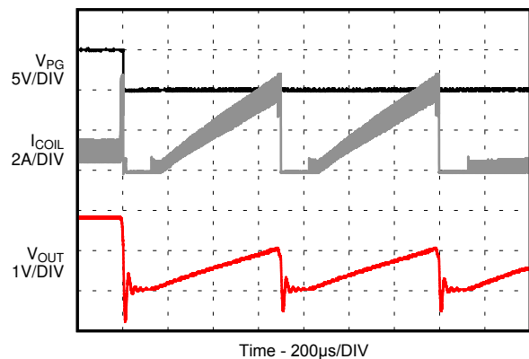
Figure 8-26. HICCUP Short Circuit Protection
