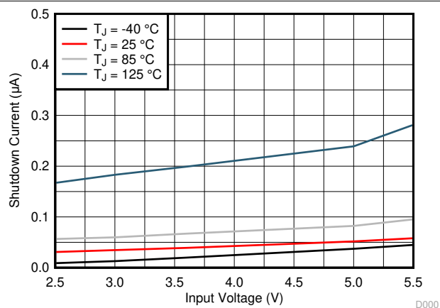
Figure 6-3. Shutdown Current
