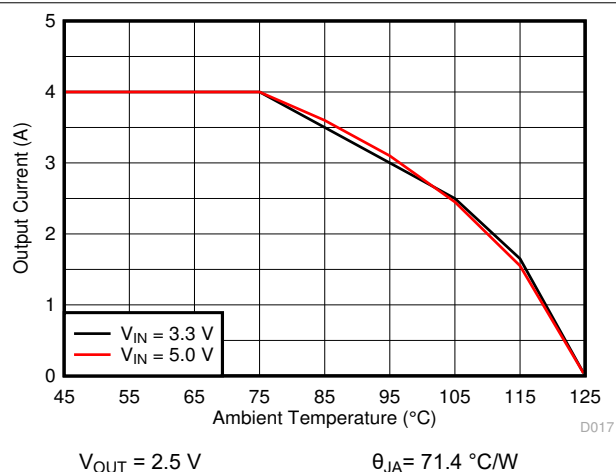
Figure 8-16. Thermal Derating
