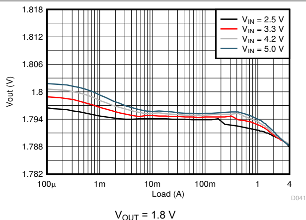
Figure 8-7. Load Regulation
