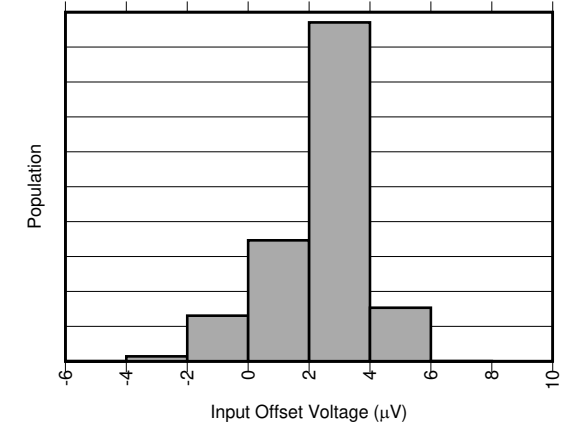
Figure 4. Input Offset Production Distribution, A4 devices
