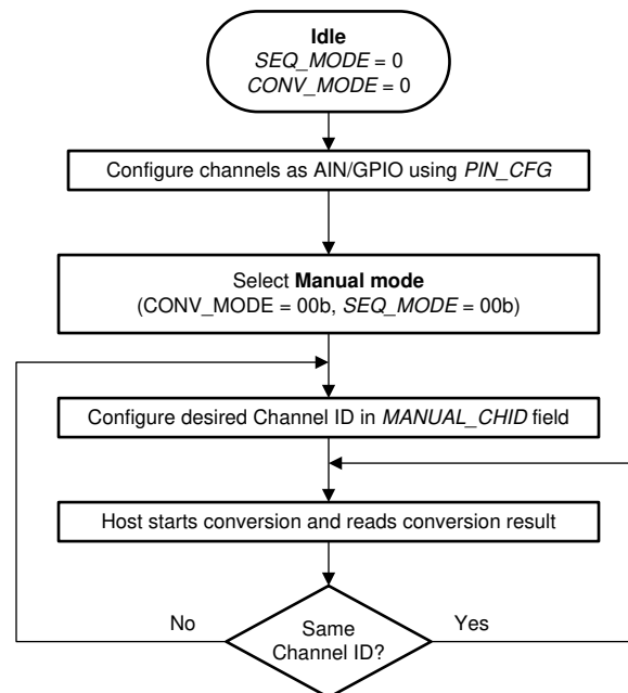
Figure 34. Device Operation in Manual Mode
