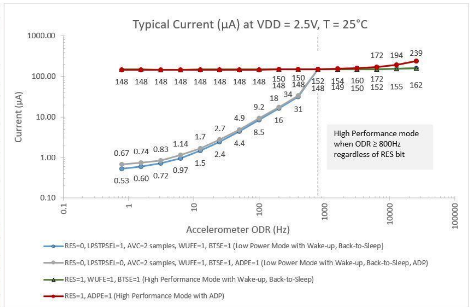
Figure 2: Current as a function of Output Data Rate (ODR) and Power Mode Settings
