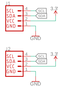
Qwiic Connectors
