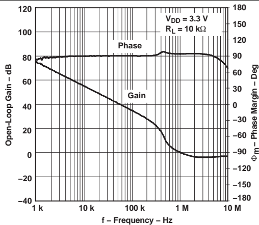
Figure 27. Open-Loop Gain and Phase Margin vs Frequency
