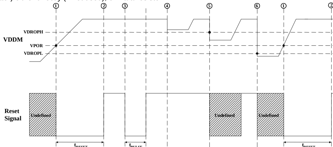
1. Device behavior is undefined until VDDM rises above VPOR, at which point internal reset procedure is started. 2. After t_{\text{RESET}} , the reset procedure is completed. 3. In operation, the SX1508QB and SX1509QB may be reset (POR like or LED driver counters only depending on RegMisc setting) at anytime by an external device driving NRESET low for t_{\text{PULSE}} or longer. Chip can be accessed normally again after NRESET rising edge. 4. During a brown-out event, if VDDM drops above VDROPH a reset will not occur. 5. During a brown-out event, if VDDM drops between VDROPH and VDROPL a reset may occur. 6. During a brown-out event, if VDDM drops below VDROPL a reset will occur next time VPOR is crossed.
