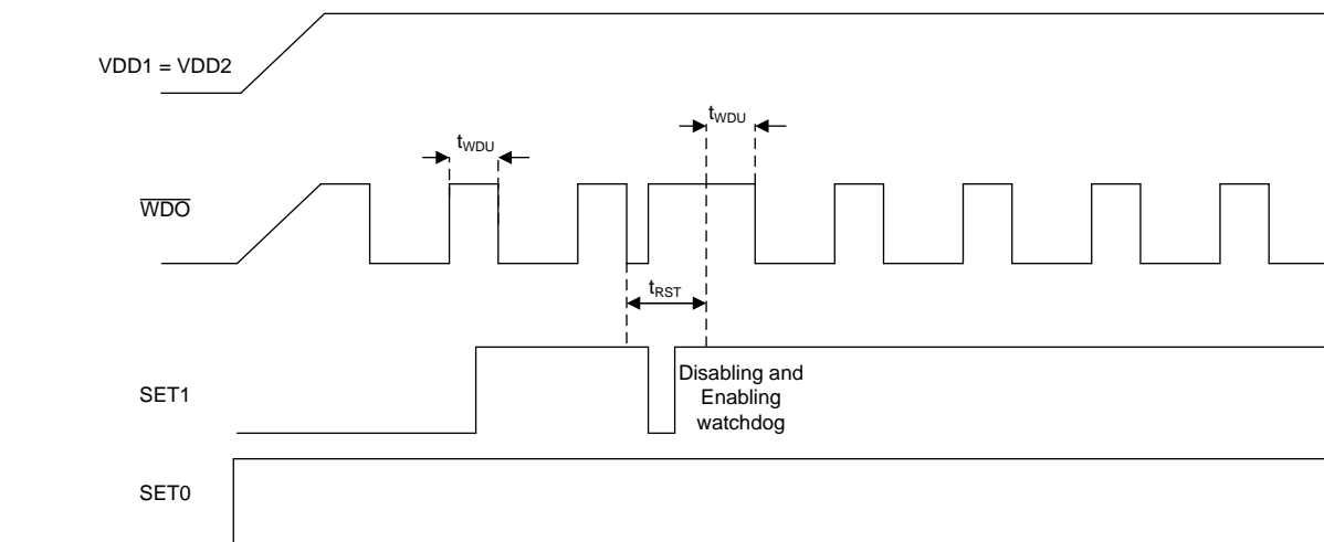
Figure 10. Enabling and Disabling the Watchdog Timer During a WDO Reset Event
