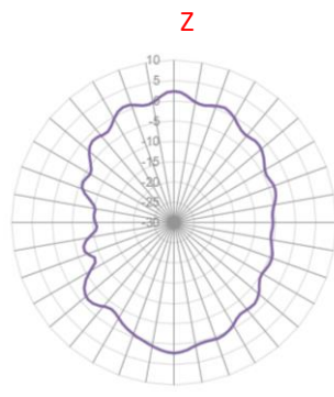
XZ Plane
