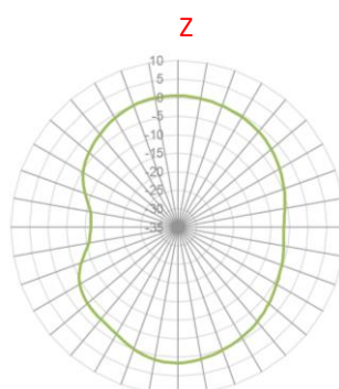
XZ Plane
