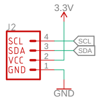
QWIIC_RIGHT_ANGLE
