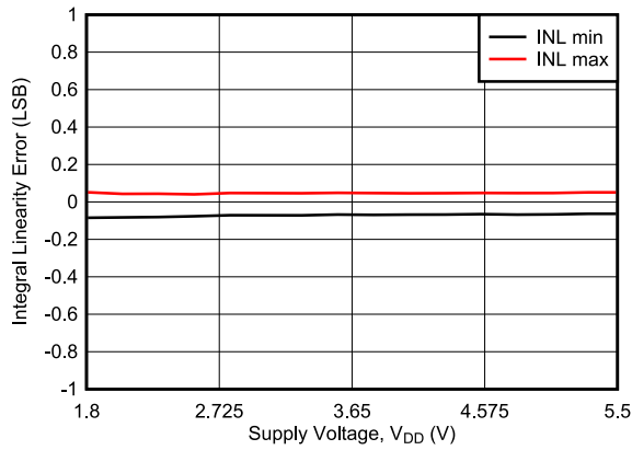
Figure 7-21. Integral Linearity Error vs Supply Voltage
