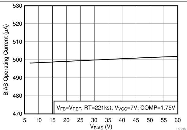
Figure 9. I_{OPERATING(BIAS)} Including RT Current vs V_{BIAS}
