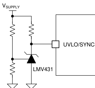
Figure 33. Inverted UVLO
