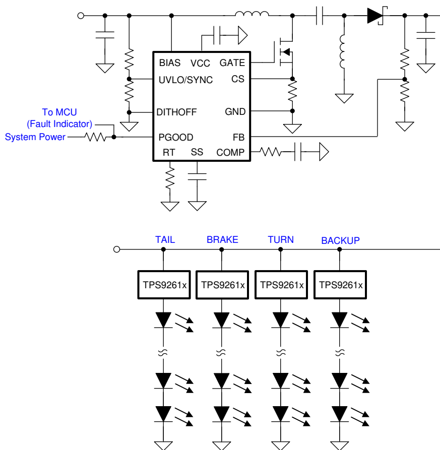
Figure 51. Dual-Stage Automotive Rear-Lights LED Driver
