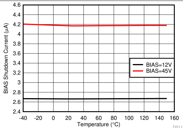
Figure 11. I_{SHUTDOWN} vs Temperature
