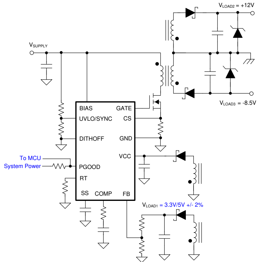
Figure 48. Primary-Side Regulated Multiple-Output Isolated Flyback
