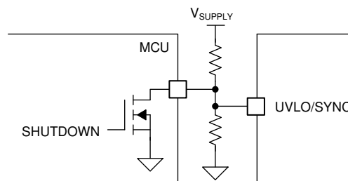
Figure 27. UVLO and Shutdown
