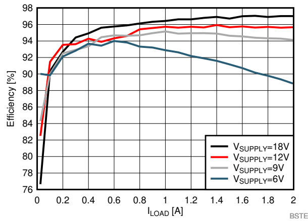
Figure 39. Efficiency
