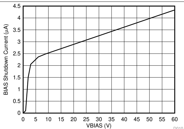
Figure 10. I_{SHUTDOWN(BIAS)} vs V_{BIAS}
