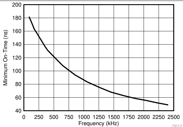
Figure 12. t_{ON(MIN)} vs Frequency
