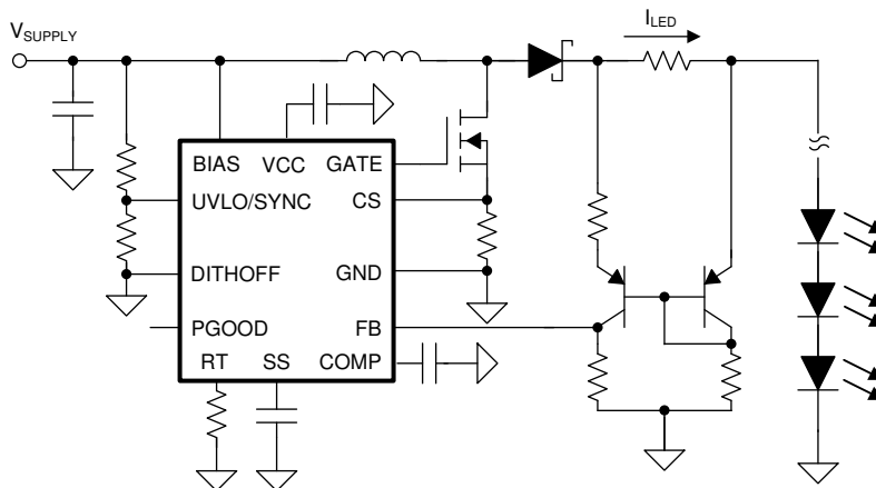
Figure 50. LED Driver with High-Side Current Sensing
