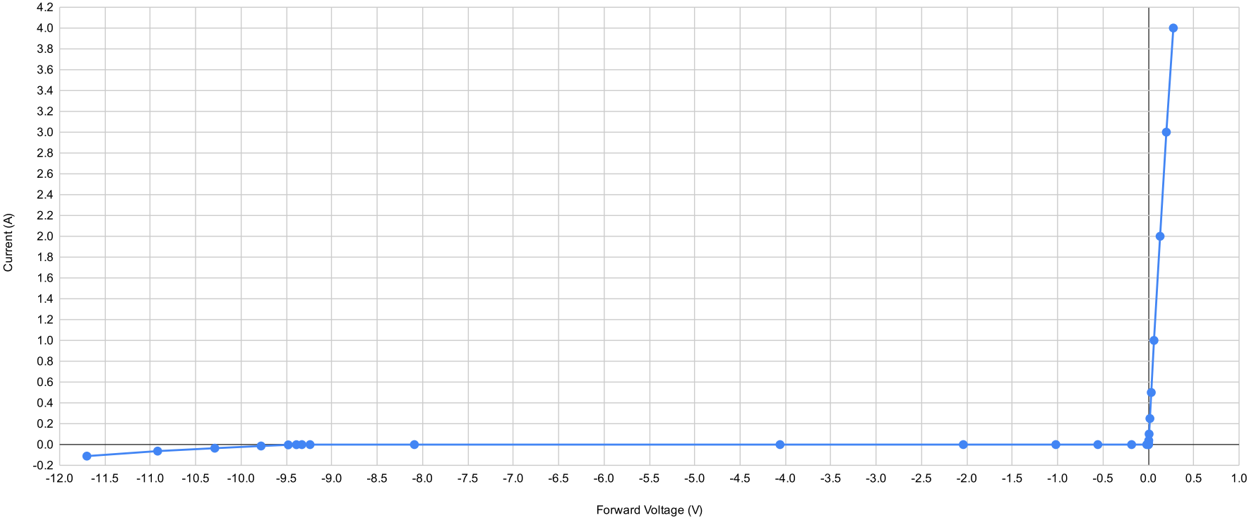
I-V Curve (VIN=20V)
