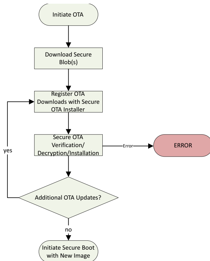
Figure 10. Secure OTA Flow
