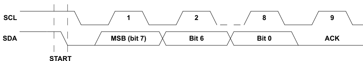
Figure 46. I 2 C Acknowledge
