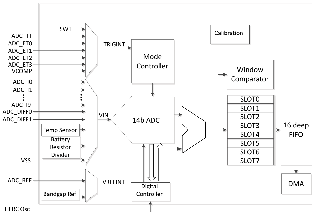
Figure 89. Block Diagram for ADC and Temperature Sensor
