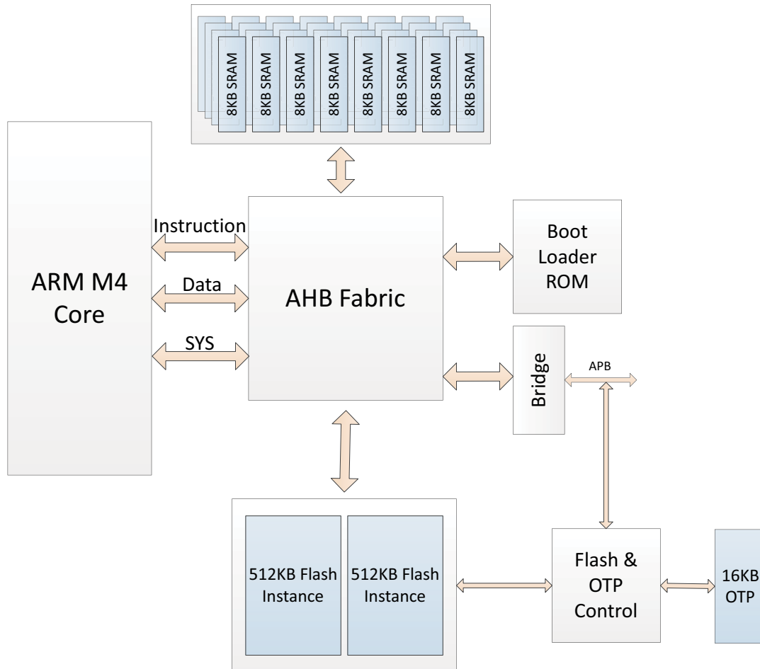
Figure 5. Block Diagram for Flash and OTP Memory Subsystem
