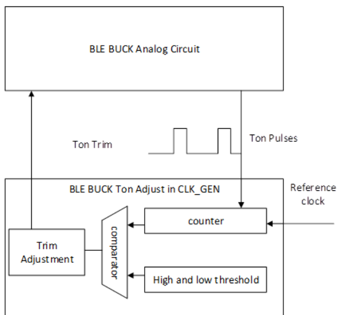
Figure 94. BLE/Burst Buck Ton Adjustment Diagram
