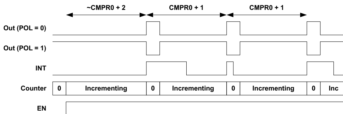
Figure 68. Counter/Timer Operation, FN = 1
