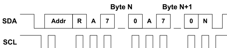
Figure 31. I 2 C Write Operation with No Address Offset
