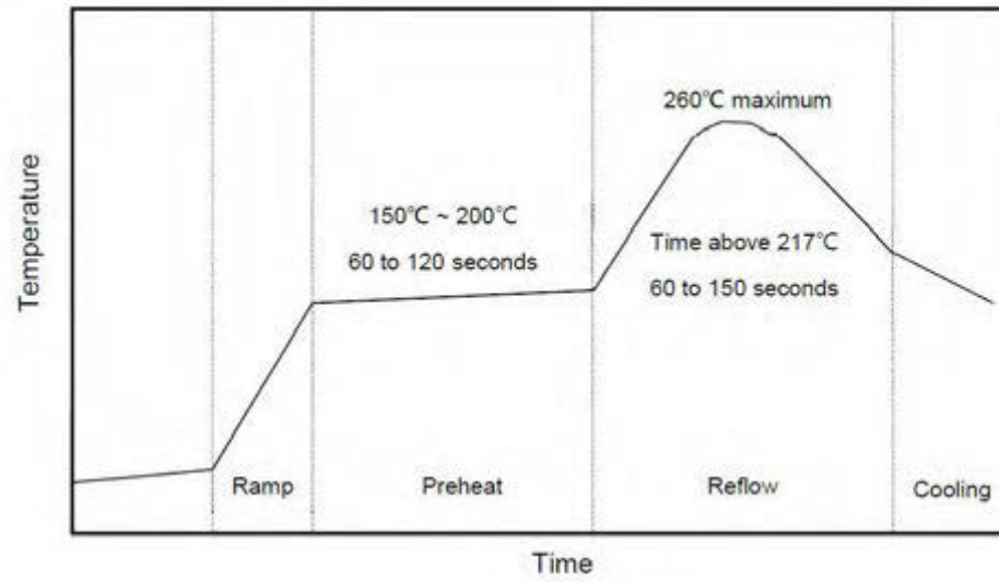
Figure 105. Reflow Profile
