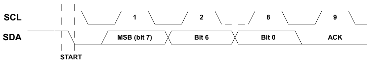
Figure 24. I 2 C Acknowledge
