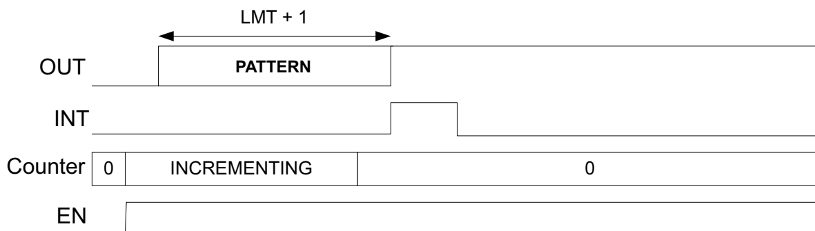
Figure 71. Counter/Timer Operation, FN = 4
