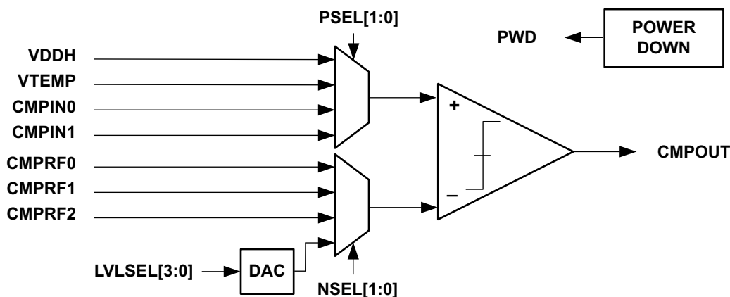
Figure 92. Block diagram for the Voltage Comparator Module
