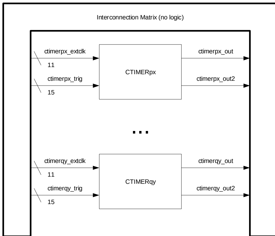
Figure 83. CTIMER Interconnection
