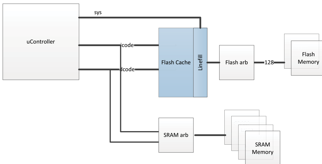
Figure 6. Block Diagram for Apollo3 Blue MCU with Flash Cache
