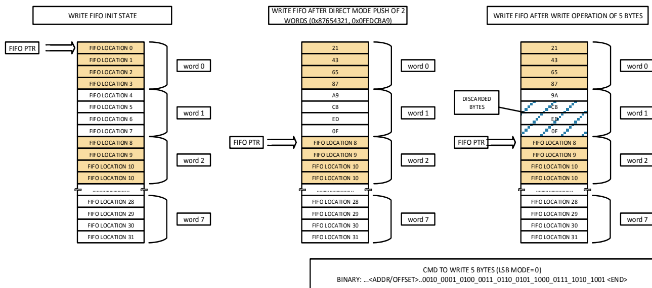
Figure 17. Direct Mode 5-byte Write Transfer
