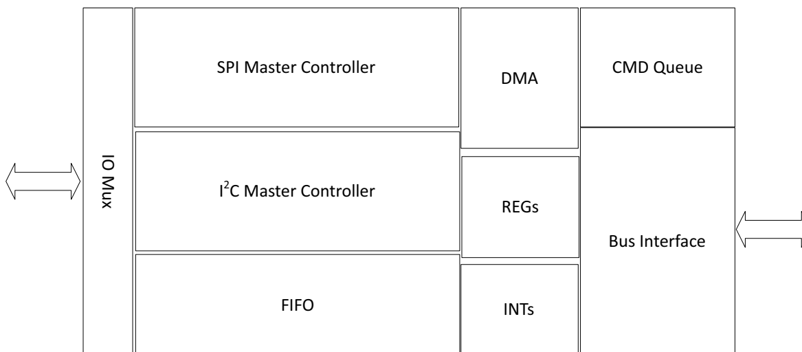
Figure 14. Block Diagram for the I 2 C/SPI Master Module
