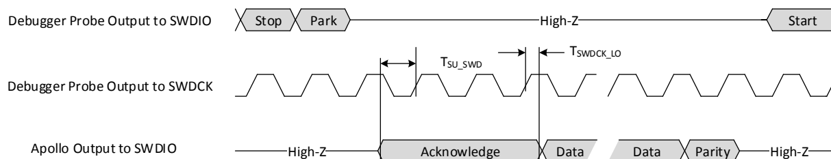
Figure 102. Serial Wire Debug Timing
