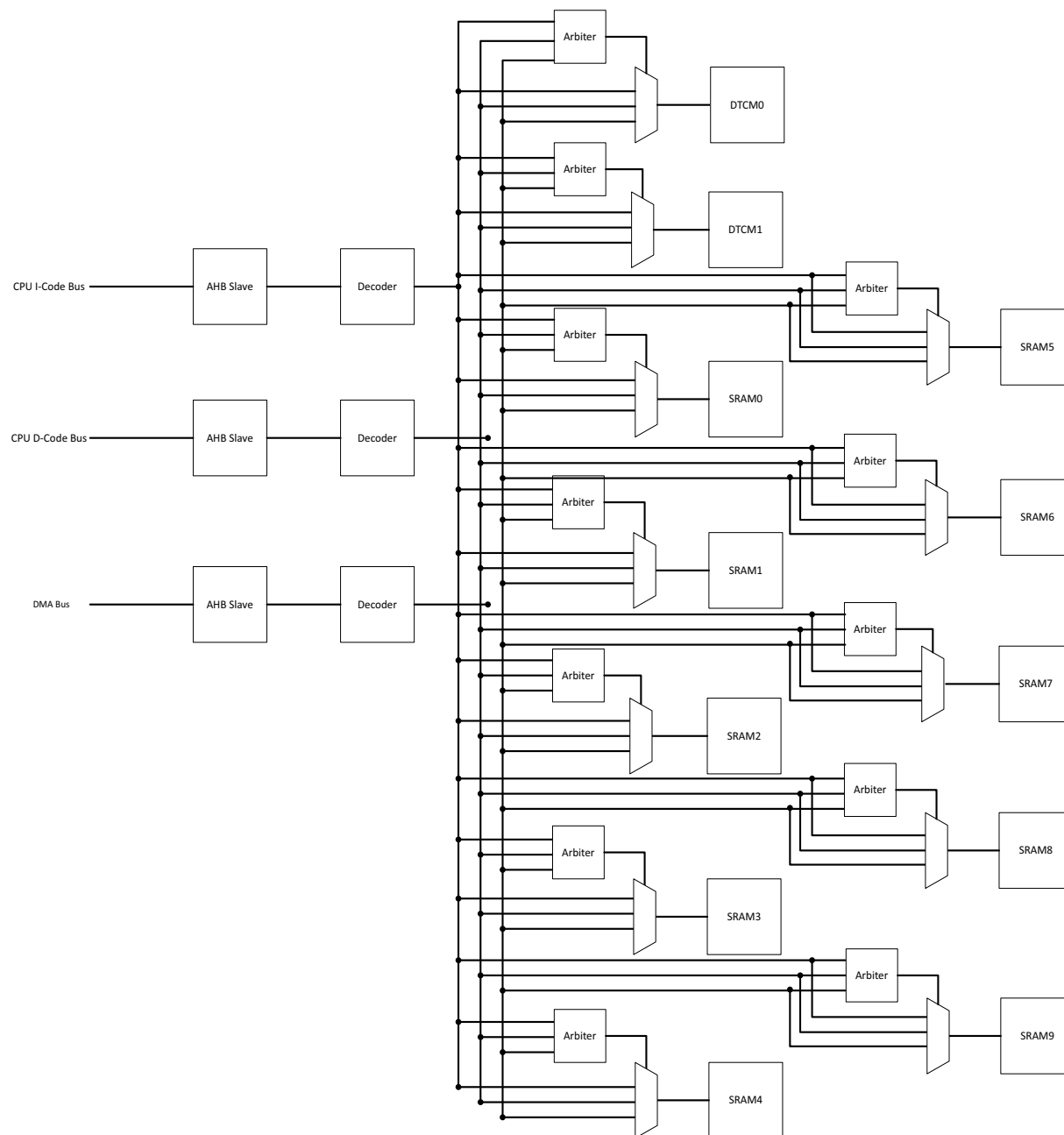
Figure 8. Block diagram for the SRAM Interface
