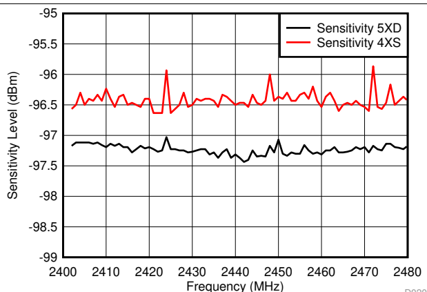
Figure 5-6. BLE Sensitivity vs Channel Frequency
