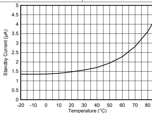
Figure 5-20. Standby Mode Supply Current vs Temperature
