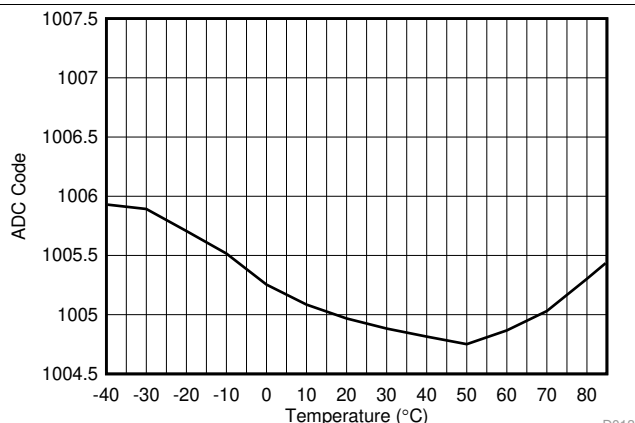
Figure 5-18. SoC ADC Output vs Temperature (Fixed Input, Internal Reference)
