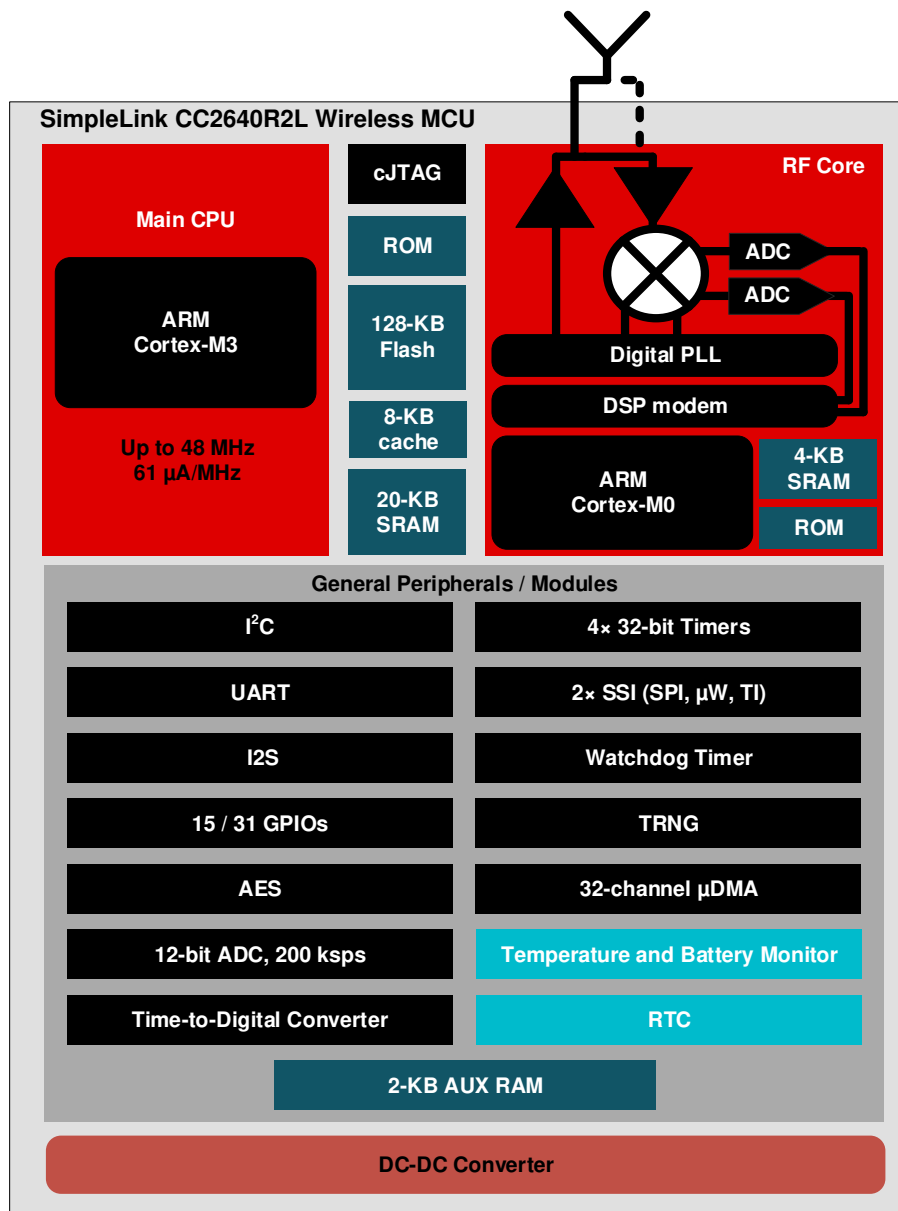
Figure 1-1. Block Diagram
