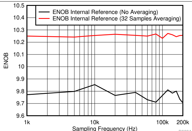
Figure 5-19. SoC ADC ENOB vs Sampling Frequency (Scaling Enabled, Input Frequency = FS / 10)
