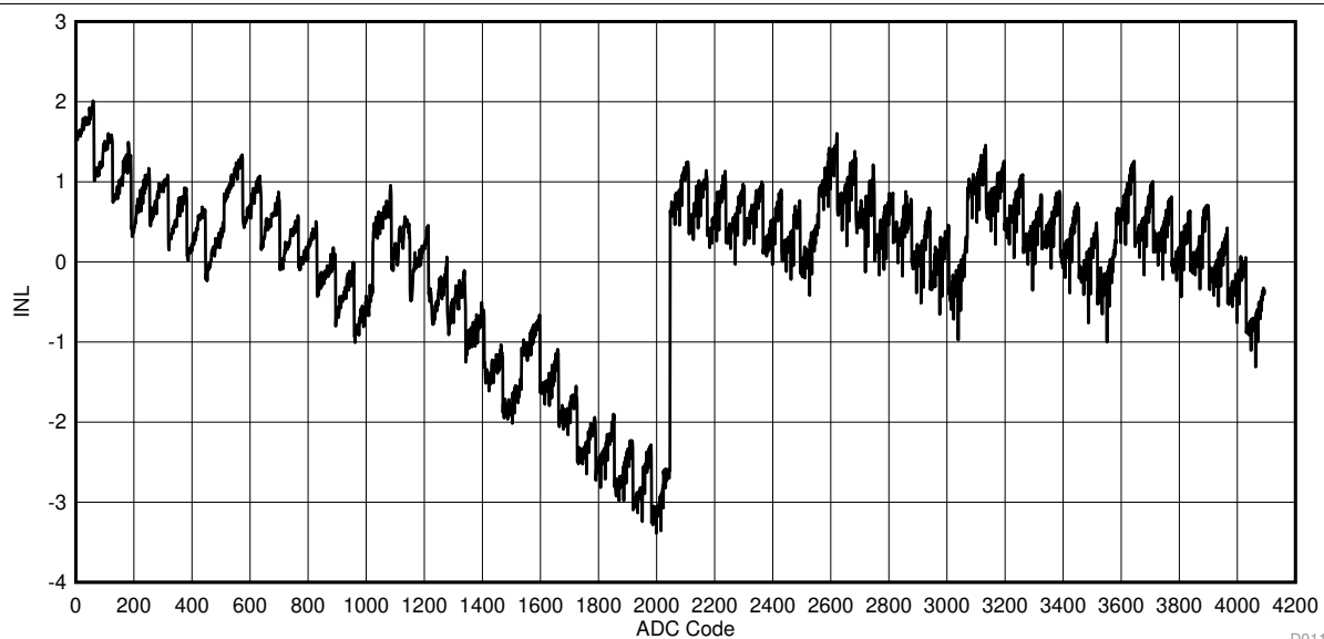
Figure 5-22. SoC ADC INL vs ADC Code (Internal Reference)
