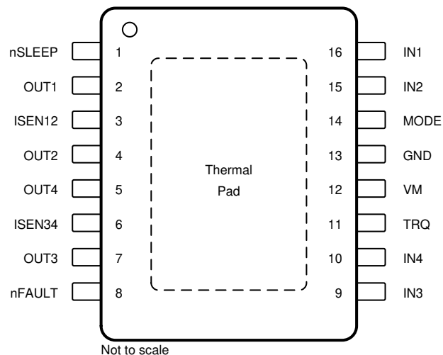
DRV8847S PW Package 16-Pin TSSOP Top View
