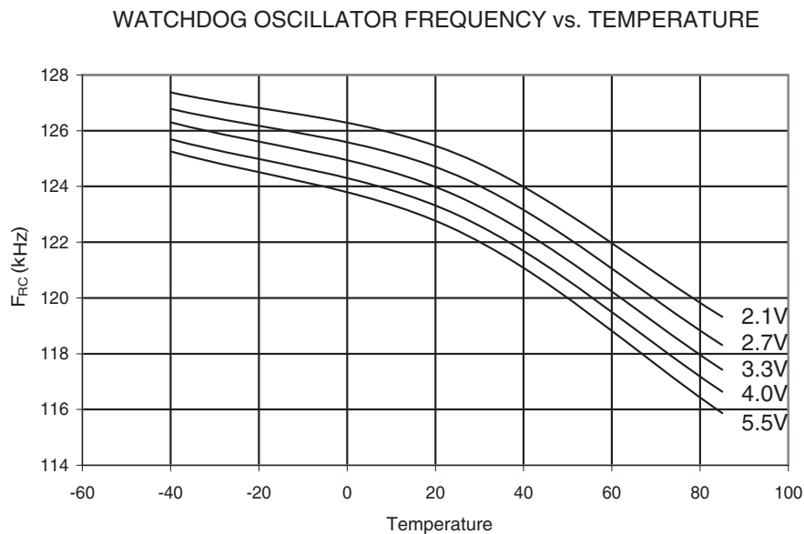
Figure 32-36. Watchdog Oscillator Frequency vs. Temperature
