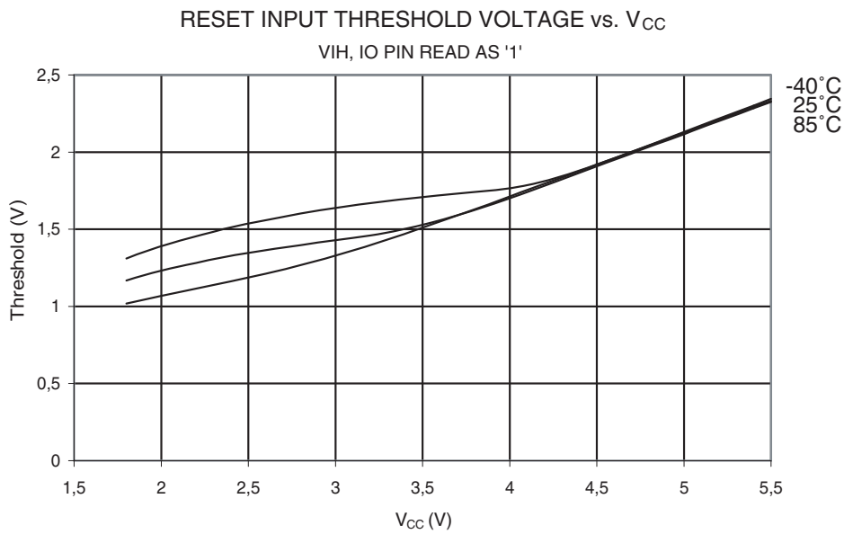
Figure 32-29. Reset Input Threshold Voltage vs. V_{CC} ( V_{IH} , IO Pin Read as "1")
