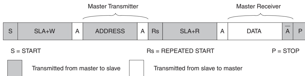
Figure 24-18. Combining Several TWI Modes to Access a Serial EEPROM
