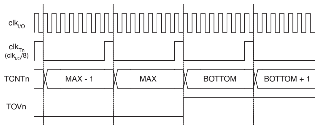
Figure 20-9. Timer/Counter Timing Diagram, with Prescaler ( f_{clk_{I/O}/8} )
