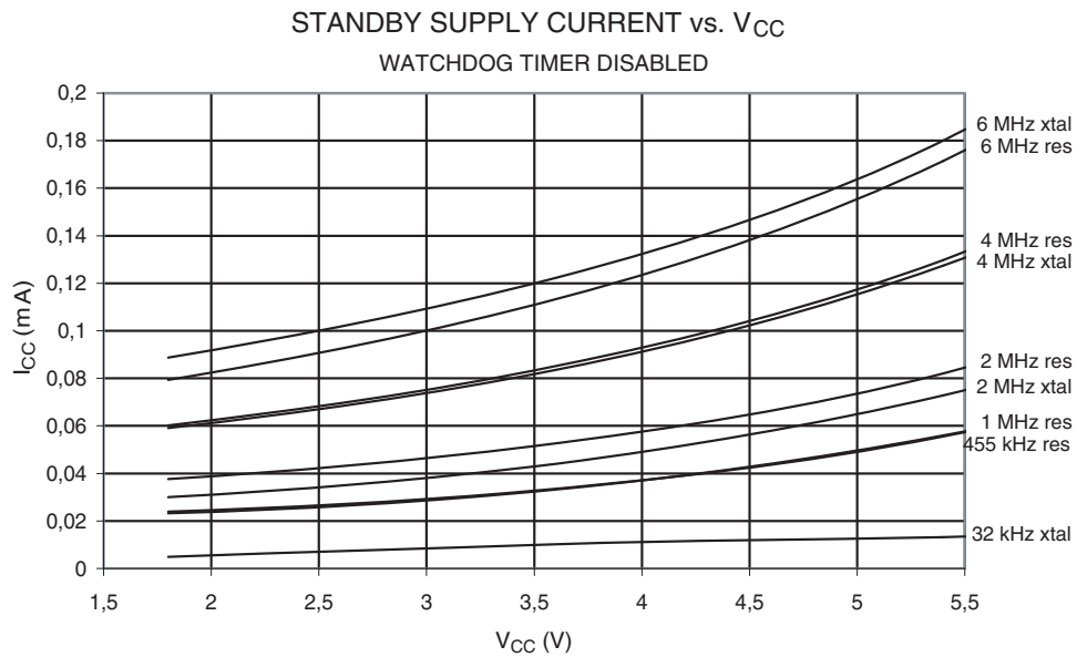
Figure 32-15. Standby Supply Current vs. V_{CC} (Watchdog Timer Disabled)
