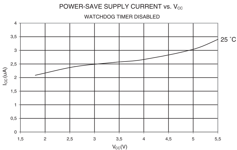
Figure 32-13. Power-save Supply Current vs. V_{CC} (Watchdog Timer Disabled)
