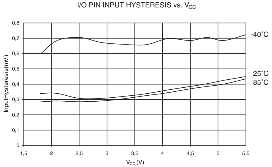
Figure 32-28. I/O Pin Input Hysteresis
