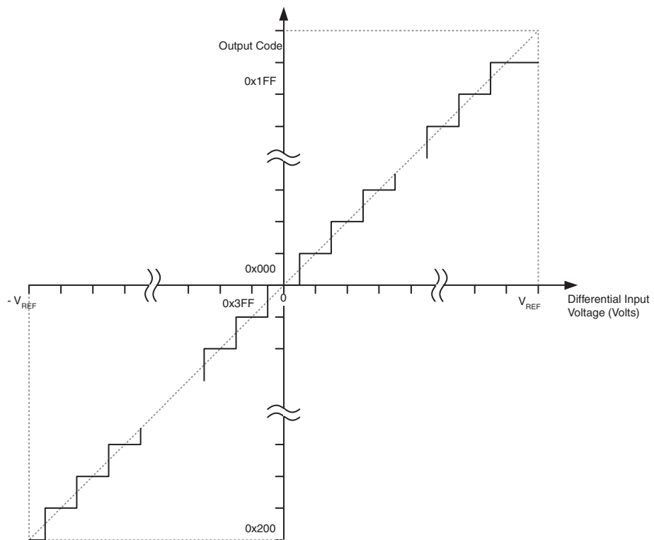
Figure 26-15. Differential Measurement Range
