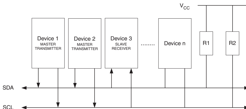
Figure 24-19. An Arbitration Example
