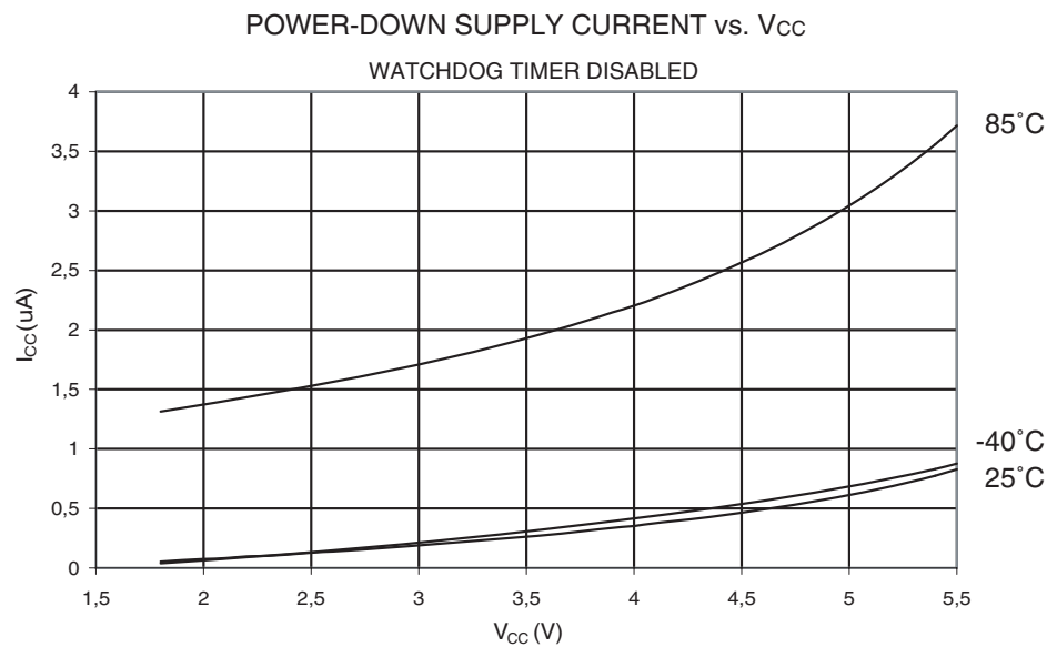
Figure 32-11. Power-down Supply Current vs. V_{CC} (Watchdog Timer Disabled)
