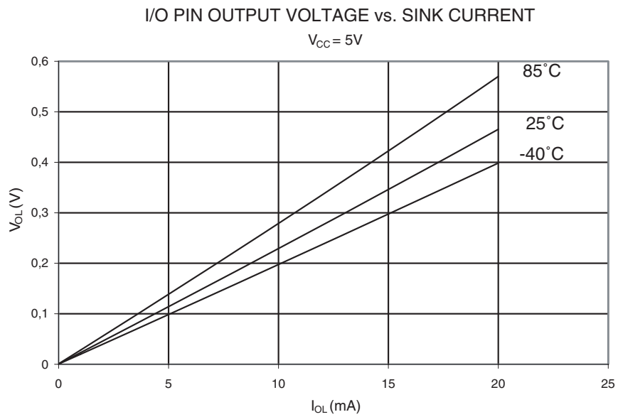
Figure 32-23. I/O Pin Output Voltage vs. Sink Current ( V_{CC} = 5\text{ V} )
