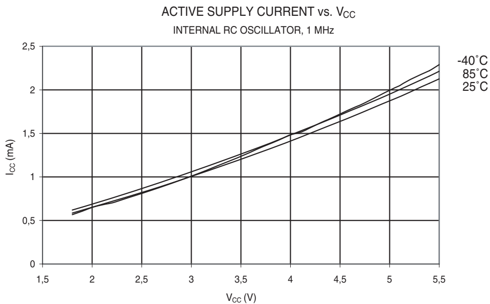
Figure 32-4. Active Supply Current vs. V_{CC} (Internal RC Oscillator, 1 MHz)
