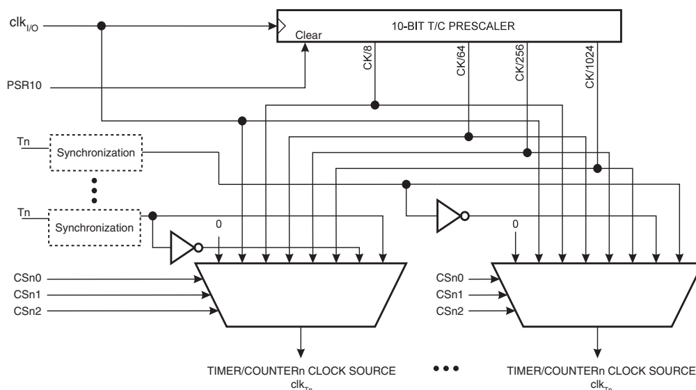
Figure 18-2. Prescaler for synchronous Timer/Counters
