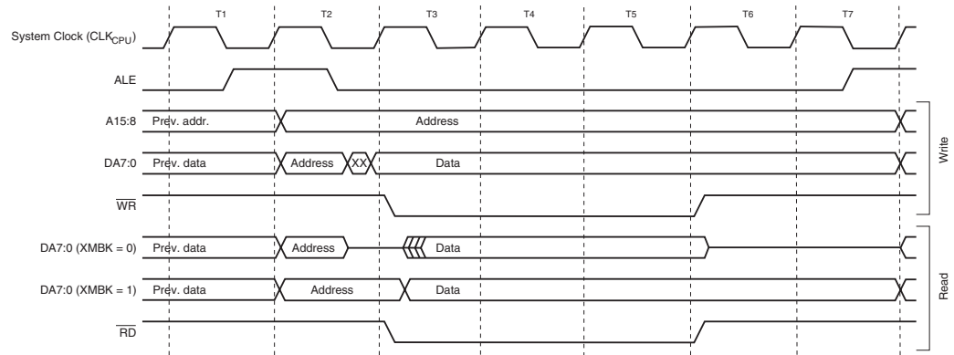
Figure 9-5. External Data Memory Cycles with SRWn1 = 1 and SRWn0 = 1 (1)
