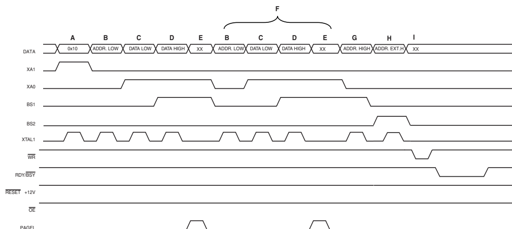
Figure 30-2. Programming the Flash Waveforms (1)
