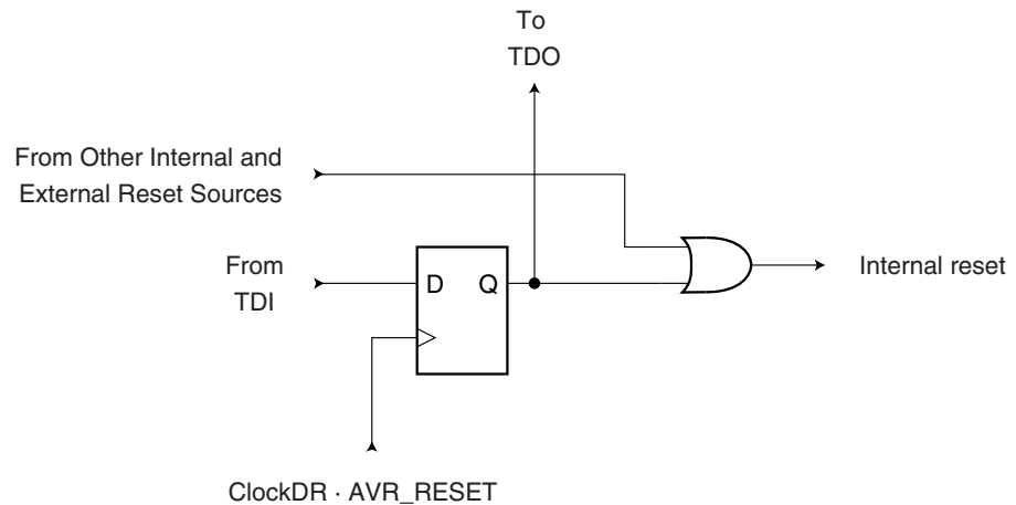
Figure 28-1. Reset Register
