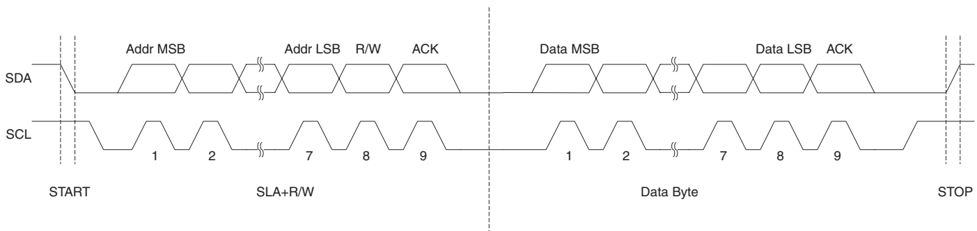
Figure 24-5. Typical Data Transmission
