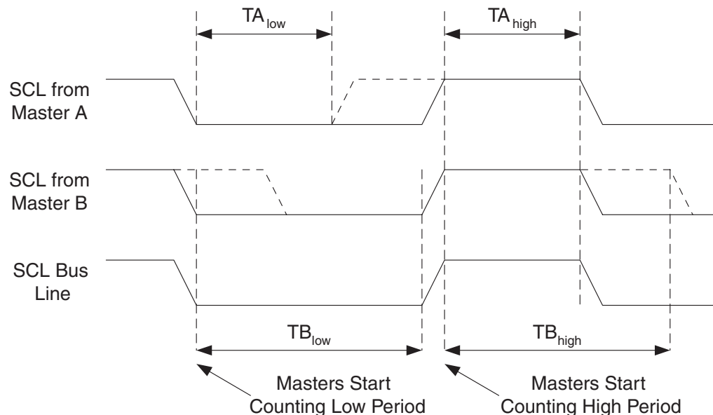
Figure 24-6. SCL Synchronization Between Multiple Masters
