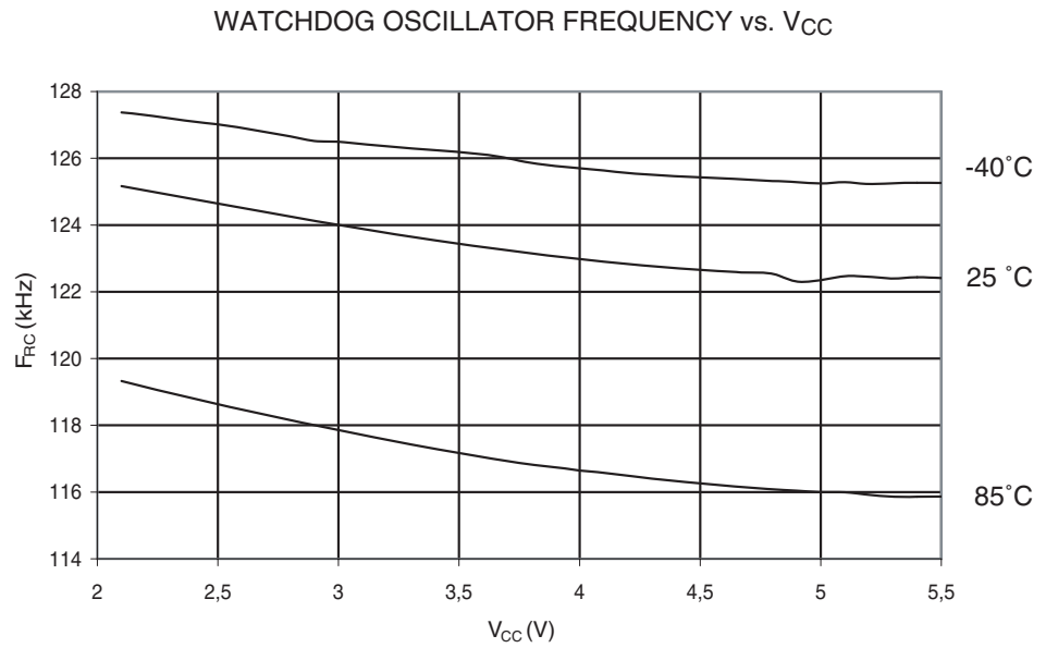
Figure 32-35. Watchdog Oscillator Frequency vs. V_{CC}
