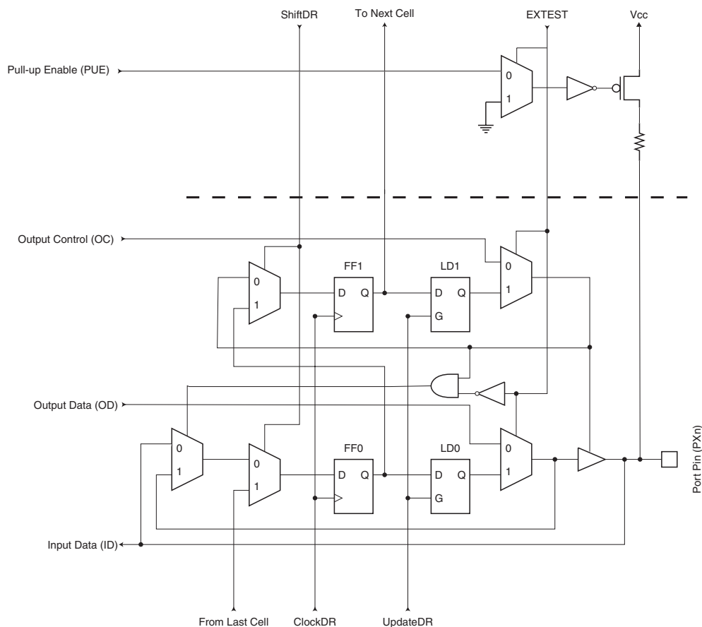
Figure 28-2. Boundary-scan Cell for Bi-directional Port Pin with Pull-up Function.
