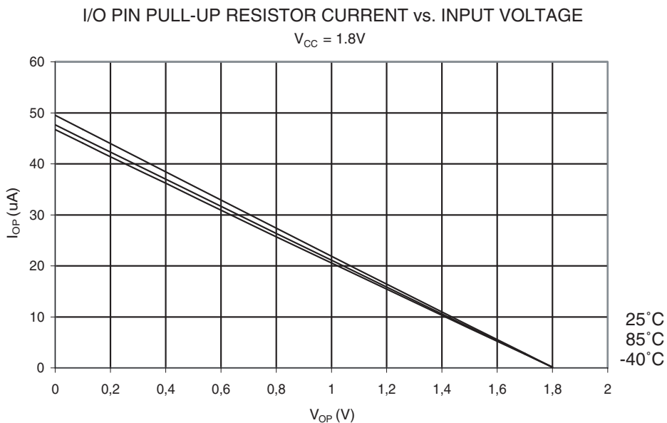
Figure 32-16. I/O Pin Pull-up Resistor Current vs. Input Voltage ( V_{CC} = 1.8\text{ V} )
