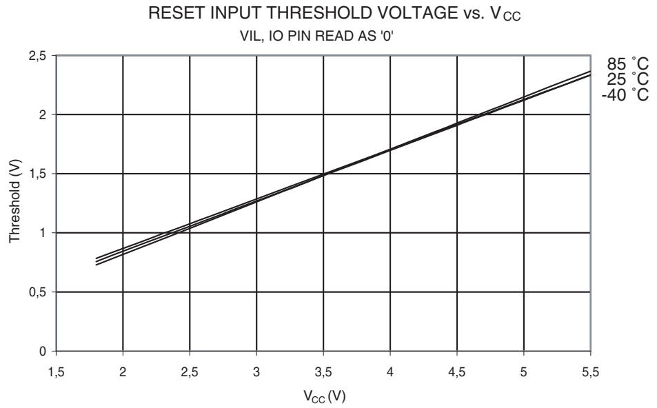
Figure 32-30. Reset Input Threshold Voltage vs. V_{CC} ( V_{IL} , IO Pin Read as "0")
