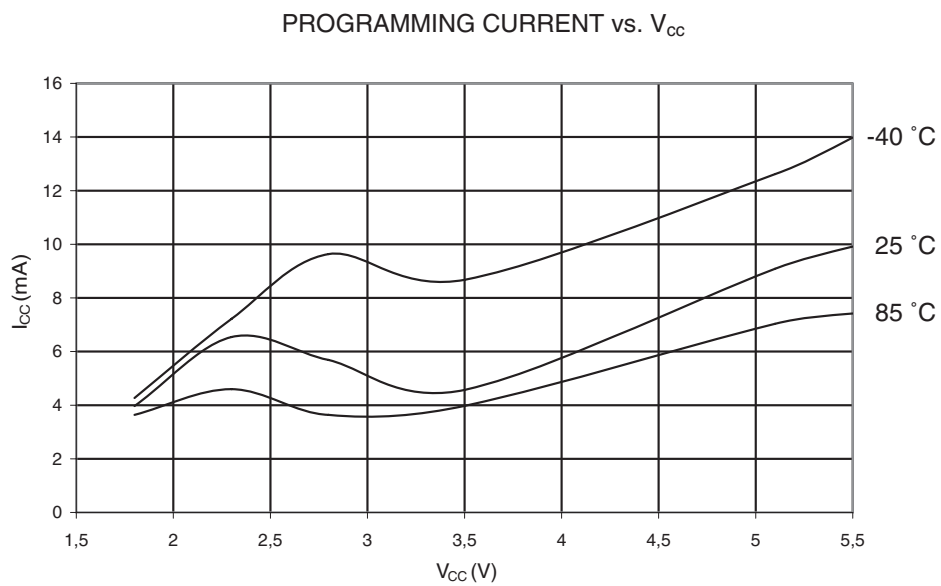
Figure 32-45. Programming Current vs. V_{CC}
