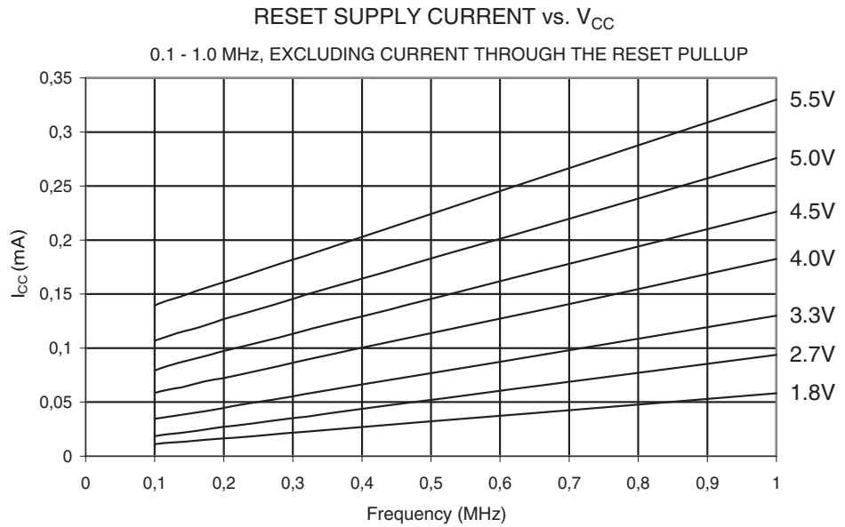
Figure 32-46. Reset Supply Current vs V_{CC} (0.1 - 1.0 MHz, Excluding Current Through The Reset Pull-up)
