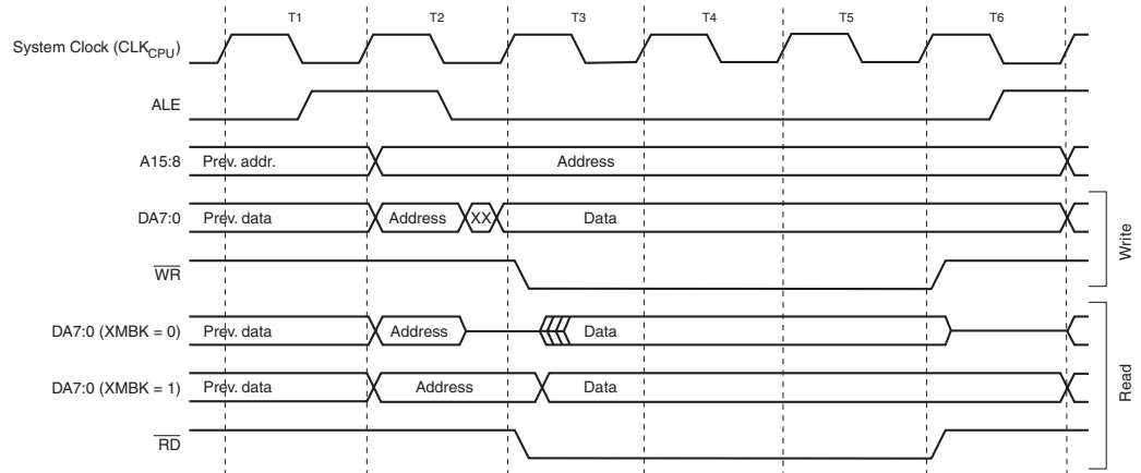
Figure 1. External Data Memory Cycles with SRWn1 = 1 and SRWn0 = 0 (1)
