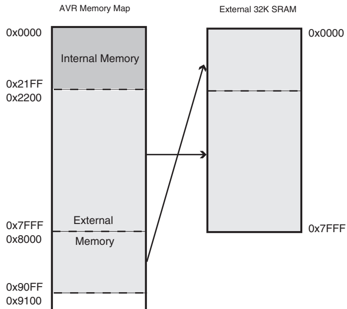
Figure 9-6. Address Map with 32 KB External Memory
