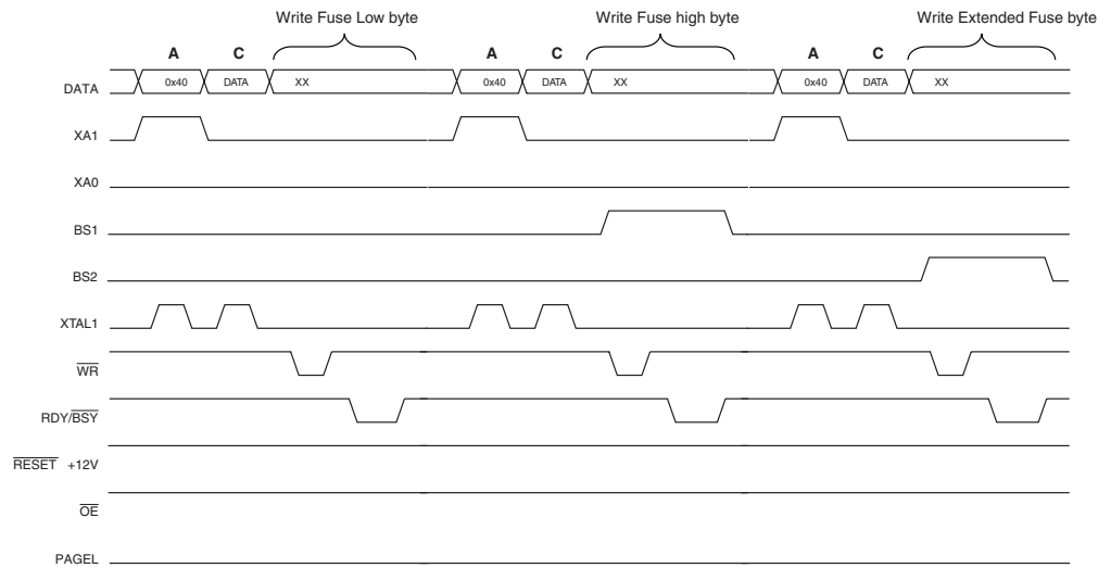
Figure 30-4. Programming the FUSES Waveforms
