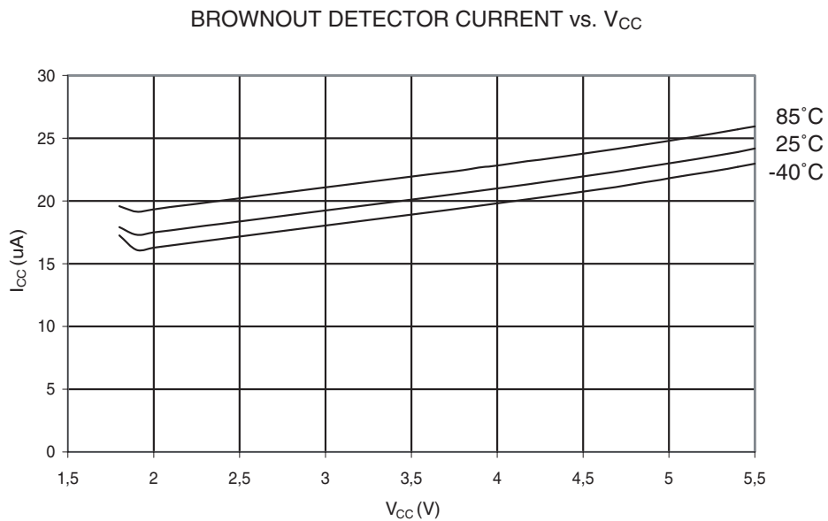
Figure 32-40. Brownout Detector Current vs. V_{CC}
