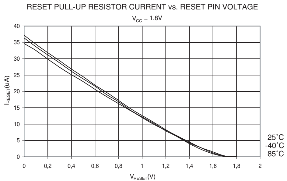
Figure 32-19. Reset Pull-up Resistor Current vs. Reset Pin Voltage ( V_{CC} = 1.8V )
