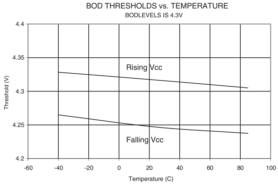
Figure 32-32. BOD Threshold vs. Temperature (BOD Level is 4.3 V)
