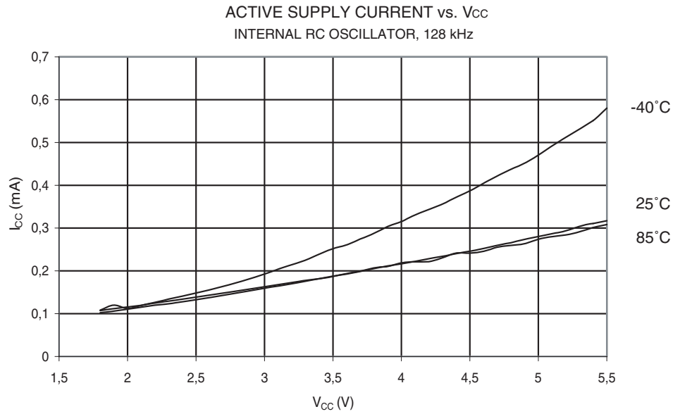
Figure 32-5. Active Supply Current vs. V_{CC} (Internal RC Oscillator, 128 kHz)
