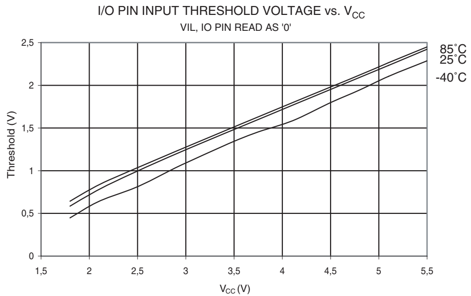
Figure 32-27. I/O Pin Input Threshold Voltage vs. V_{CC} ( V_{IL} , IO Pin Read as "0")
