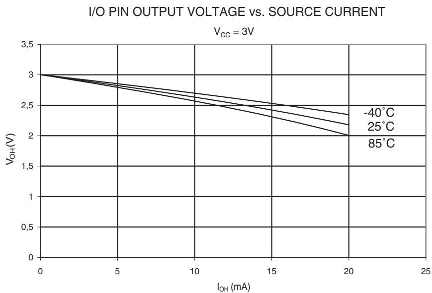
Figure 32-24. I/O Pin Output Voltage vs. Source Current ( V_{CC} = 3\text{ V} )
