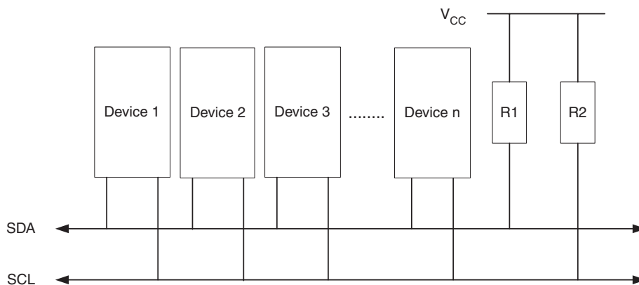
Figure 2. TWI Bus Interconnection
