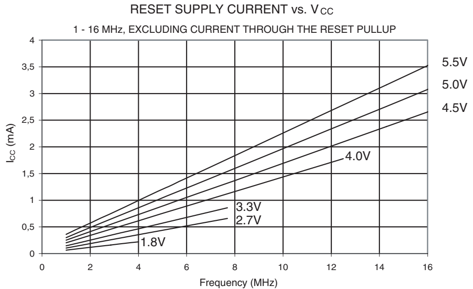
Figure 32-47. Reset Supply Current vs. V_{CC} (1 - 16 MHz, Excluding Current Through The Reset Pull-up)
