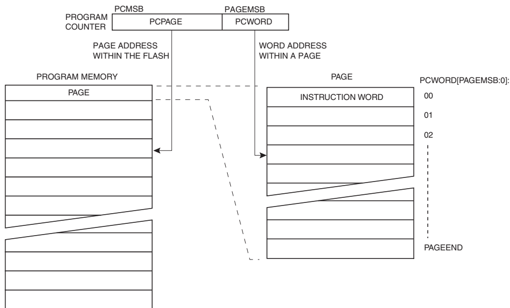
Figure 4. Addressing the Flash Which is Organized in Pages (Note:)
