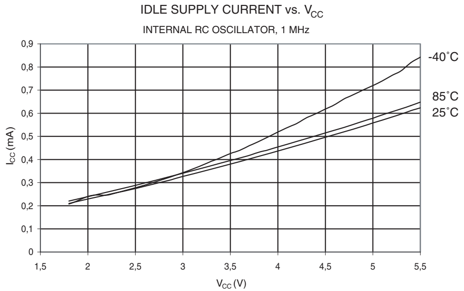
Figure 32-9. Idle Supply Current vs. V_{CC} (Internal RC Oscillator, 1 MHz)
