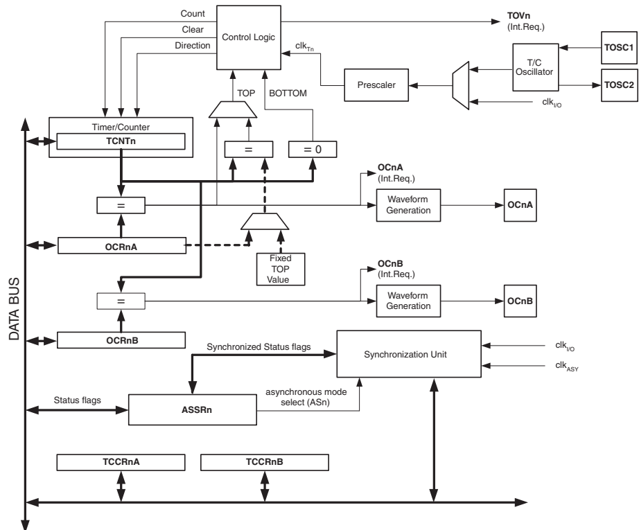
Figure 20-1. 8-bit Timer/Counter Block Diagram
