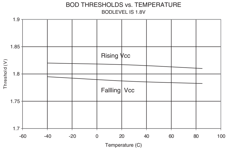
Figure 32-34. BOD Threshold vs. Temperature (BOD Level is 1.8 V)
