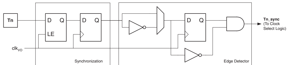
Figure 18-1. T n /T 0 Pin Sampling
