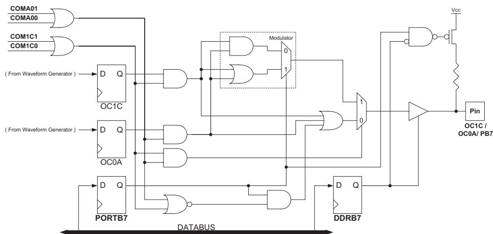
Figure 19-2. Output Compare Modulator, Schematic
