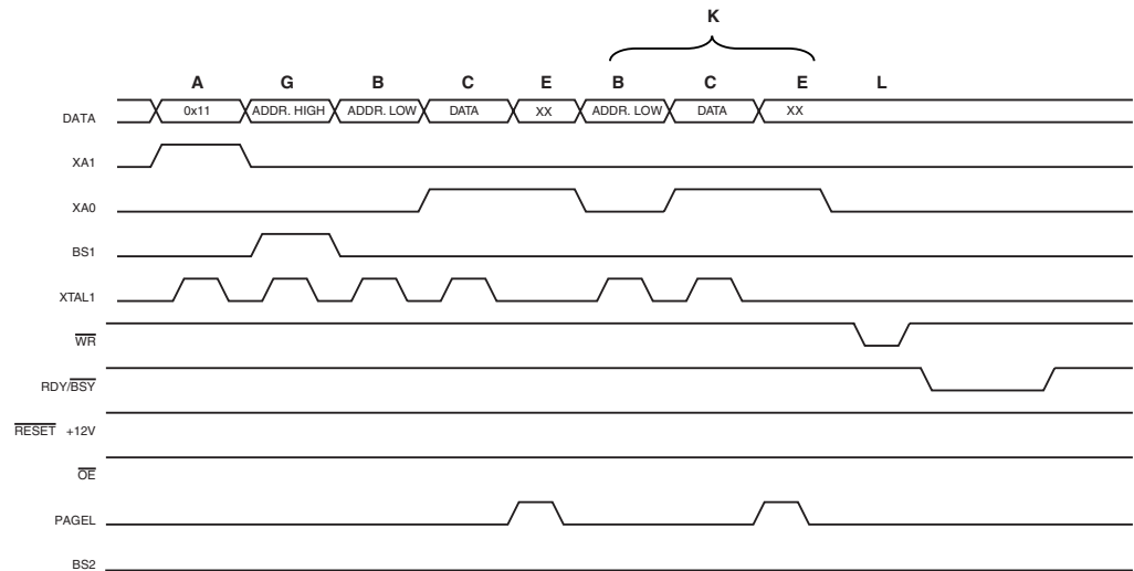
Figure 30-3. Programming the EEPROM Waveforms
