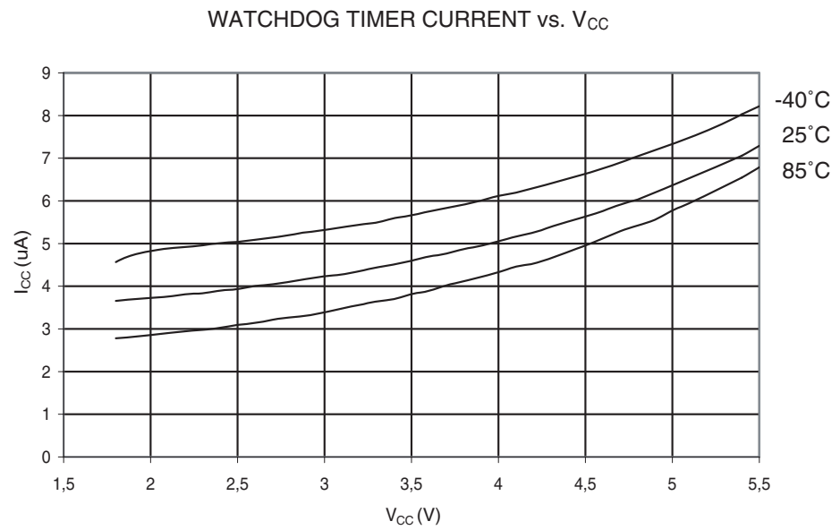
Figure 32-43. Watchdog Timer Current vs. V_{CC}
