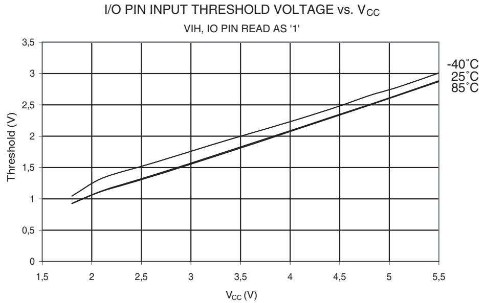
Figure 32-26. I/O Pin Input Threshold Voltage vs. V_{CC} ( V_{IH} , IO Pin Read as "1")
