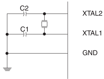
Figure 10-3. Crystal Oscillator Connections
