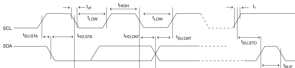
Figure 31-6. 2-wire Serial Bus Timing
