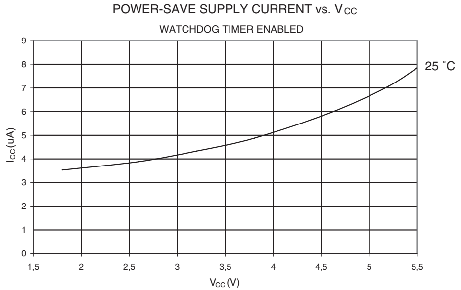
Figure 32-14. Power-save Supply Current vs. V_{CC} (Watchdog Timer Enabled)
