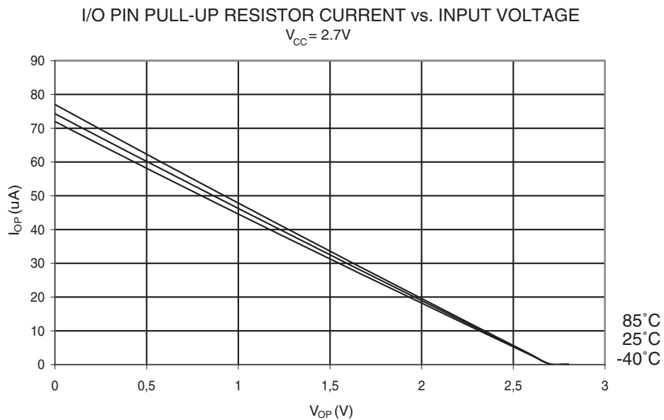
Figure 32-17. I/O Pin Pull-up Resistor Current vs. Input Voltage ( V_{CC} = 2.7\text{ V} )
