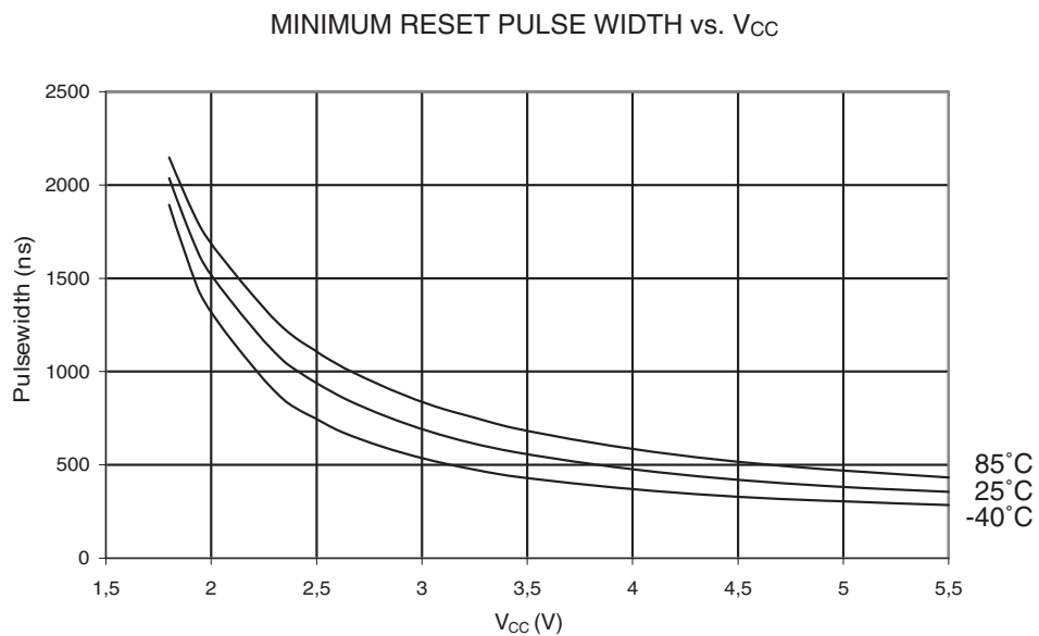
Figure 32-48. Minimum Reset Pulse Width vs. V_{CC}
