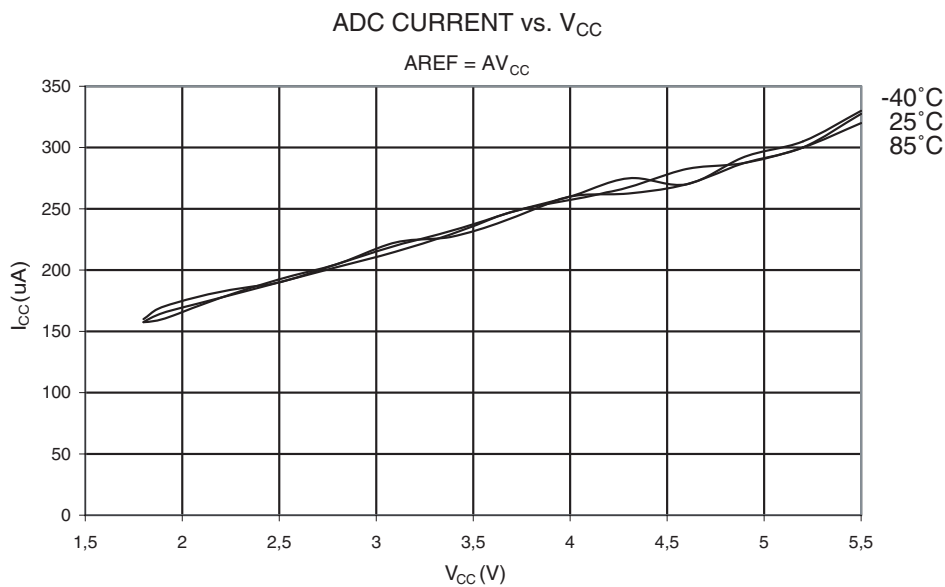
Figure 32-41. ADC Current vs. V_{CC} ( A_{REF} = AV_{CC} )
