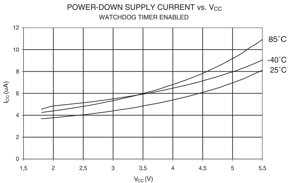
Figure 32-12. Power-down Supply Current vs. V_{CC} (Watchdog Timer Enabled)
