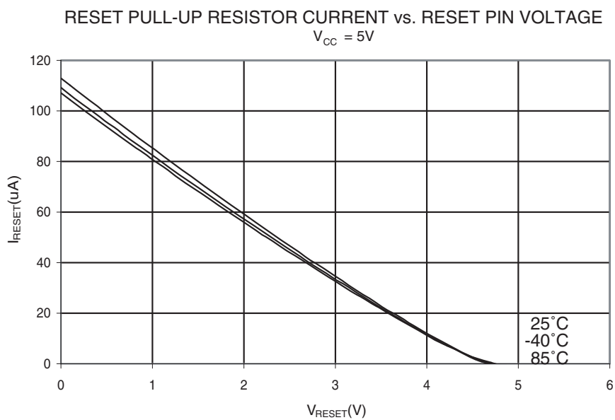
Figure 32-21. Reset Pull-up Resistor Current vs. Reset Pin Voltage ( V_{CC} = 5\text{ V} )
