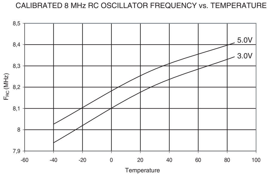
Figure 32-38. Calibrated 8 MHz RC Oscillator Frequency vs. Temperature
