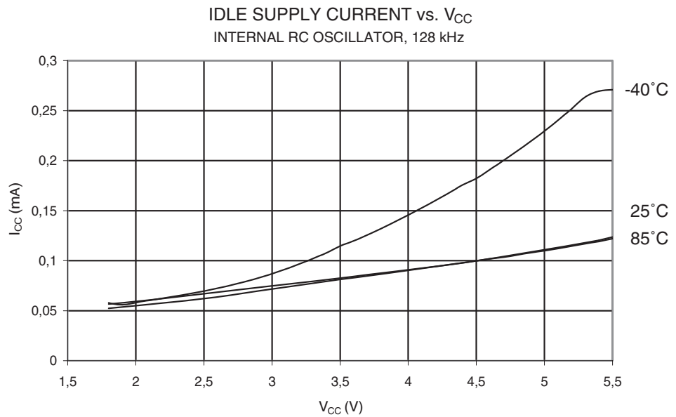
Figure 32-10. Idle Supply Current vs. V_{CC} (Internal RC Oscillator, 128 kHz)
