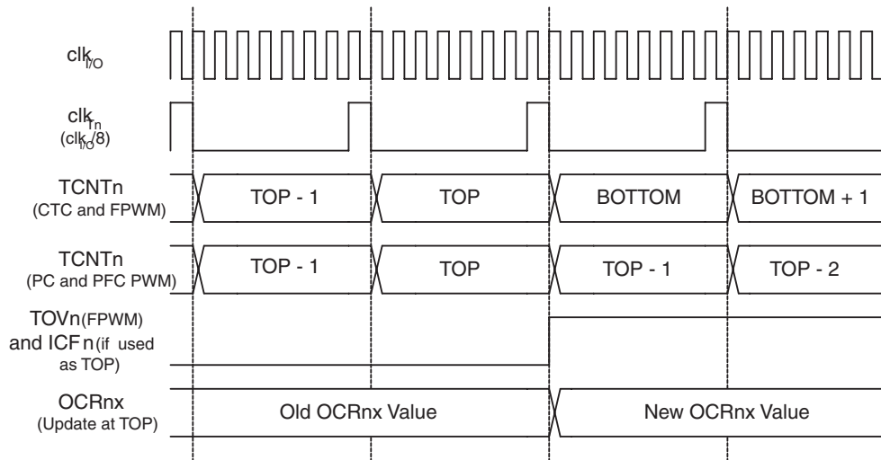
Figure 17-12. Timer/Counter Timing Diagram, with Prescaler ( f_{clk_{I/O}}/8 )
