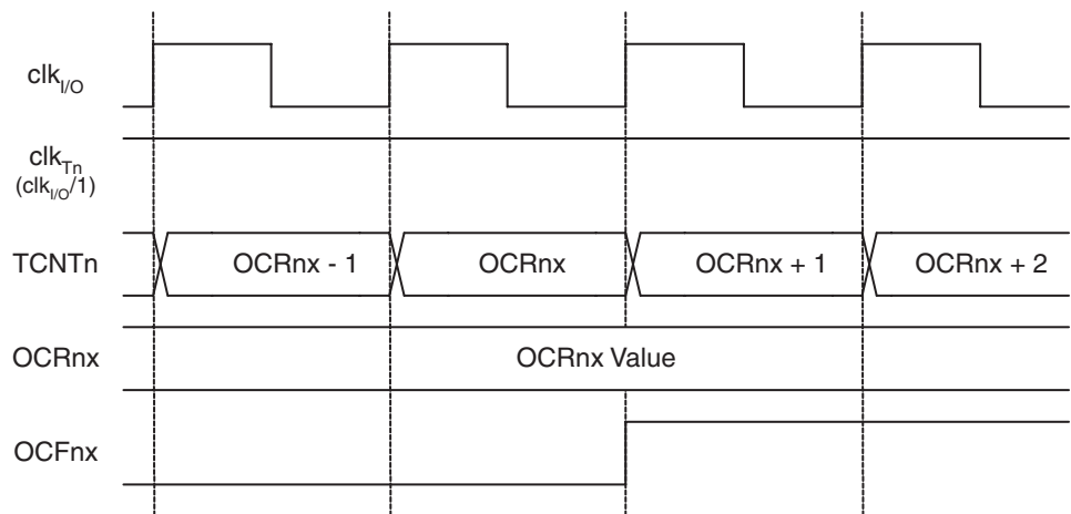
Figure 17-9. Timer/Counter Timing Diagram, Setting of OCFnx, no Prescaling
