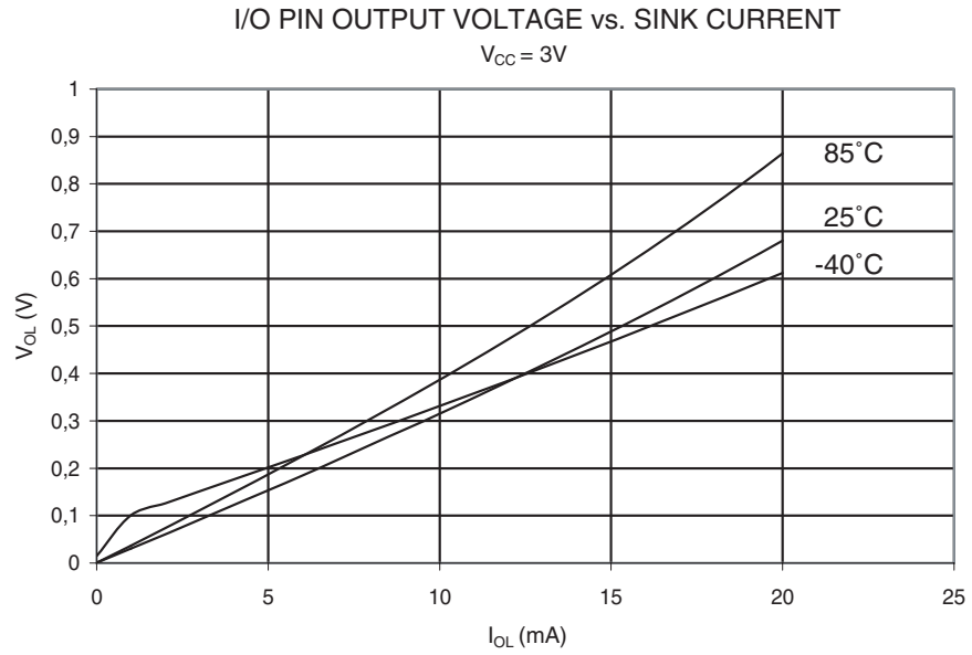
Figure 32-22. I/O Pin output Voltage vs. Sink Current ( V_{CC} = 3\text{ V} )
