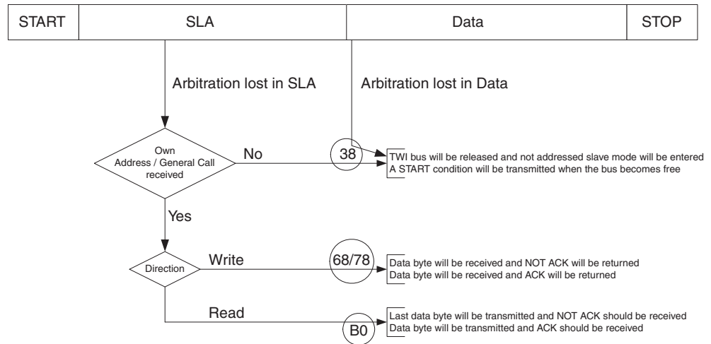
Figure 24-20. Possible Status Codes Caused by Arbitration
