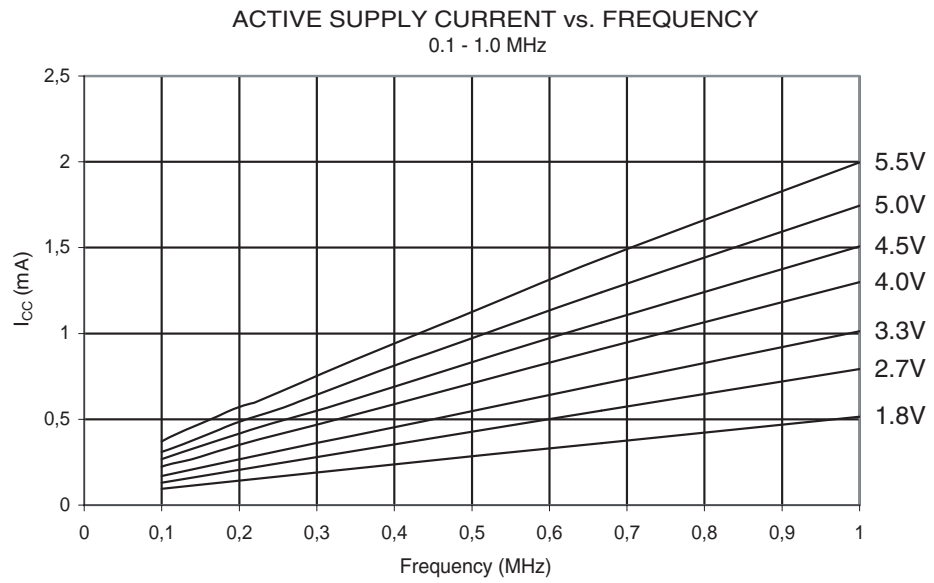
Figure 32-1. Active Supply Current vs. frequency (0.1 - 1.0 MHz)
