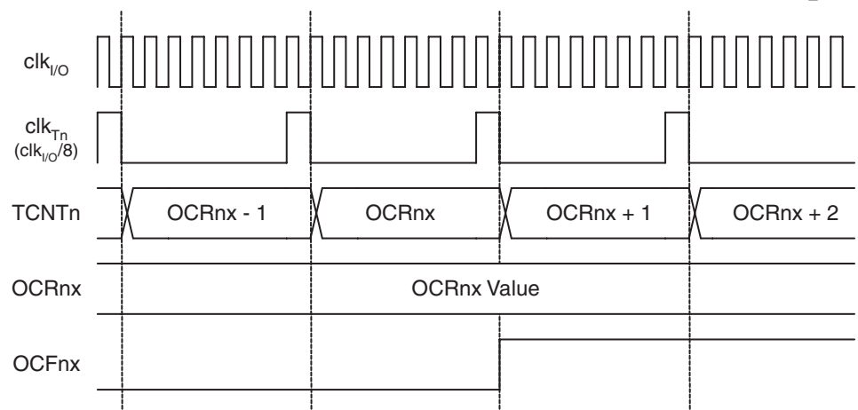
Figure 17-10. Timer/Counter Timing Diagram, Setting of OCFnx, with Prescaler ( f_{clk\_I/O}/8 )
