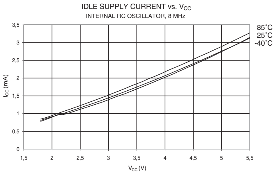
Figure 32-8. Idle Supply Current vs. V_{CC} (Internal RC Oscillator, 8 MHz)
