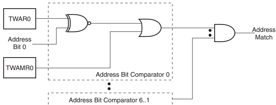
Figure 24-21. TWI Address Match Logic, Block Diagram
