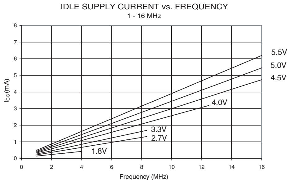
Figure 32-7. Idle Supply Current vs. Frequency (1 - 16 MHz)
