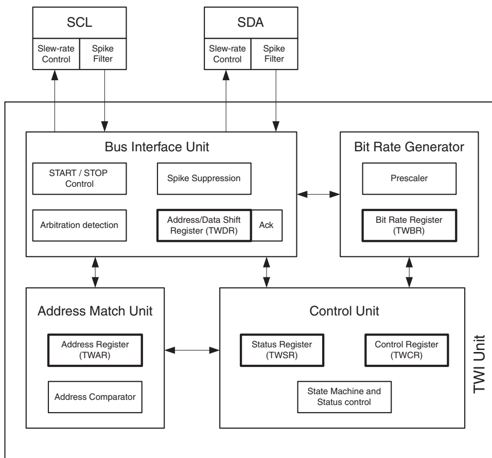
Figure 24-8. Overview of the TWI Module
