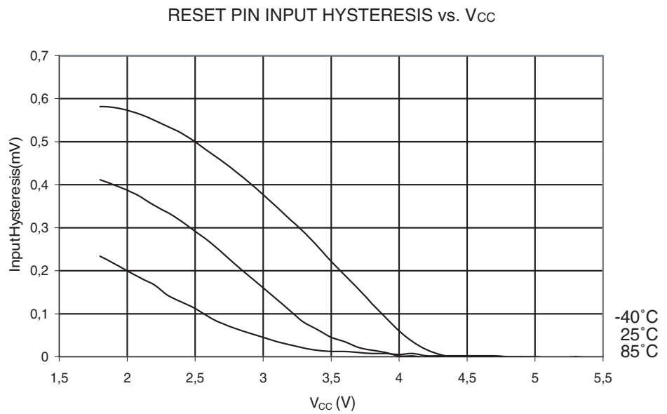
Figure 32-31. Reset Pin Input Hysteresis vs. V_{CC}
