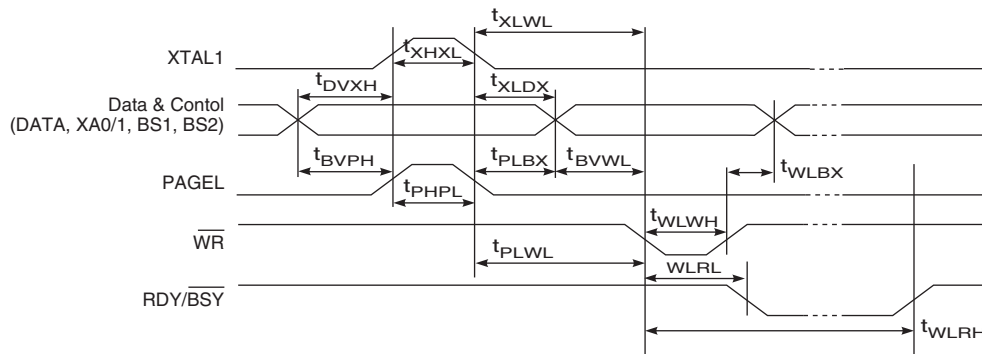
Figure 30-6. Parallel Programming Timing, Including some General Timing Requirements
