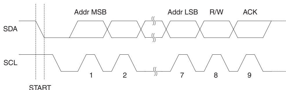
Figure 24-3. Address Packet Format
