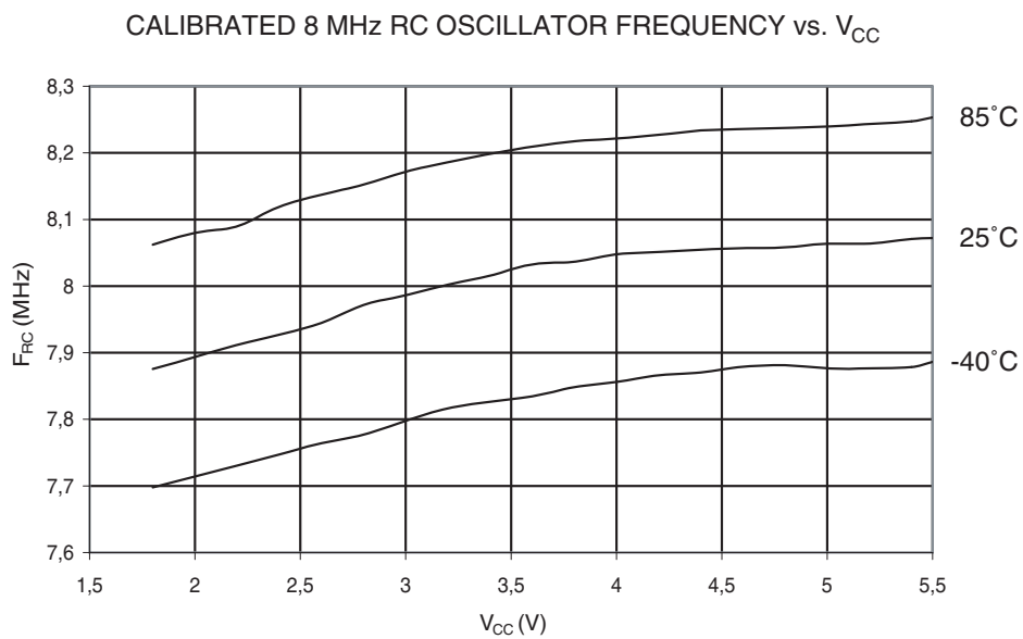
Figure 32-37. Calibrated 8 MHz RC Oscillator Frequency vs. V_{CC}
