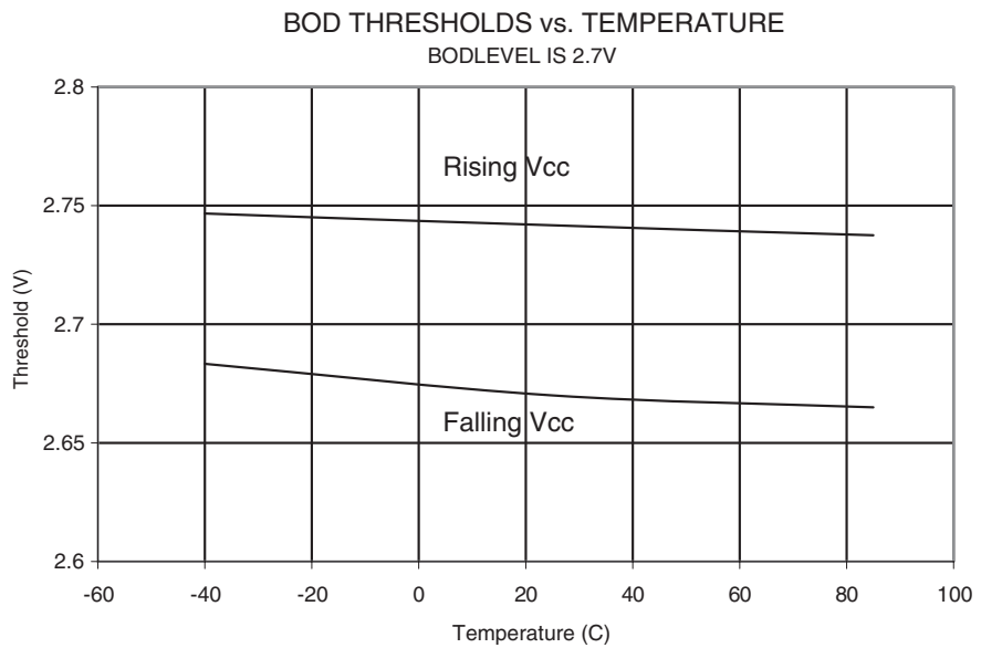
Figure 32-33. BOD Threshold vs. Temperature (BOD Level is 2.7 V)
