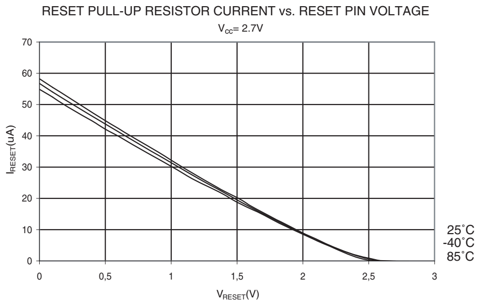
Figure 32-20. Reset pull-up Resistor Current vs. Reset Pin Voltage ( V_{CC} = 2.7\text{ V} )
