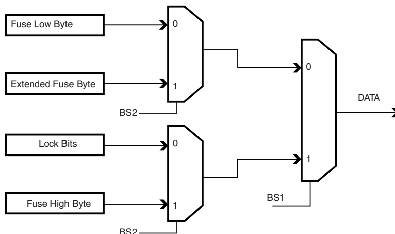
Figure 30-5. Mapping Between BS1, BS2 and the Fuse and Lock Bits During Read
