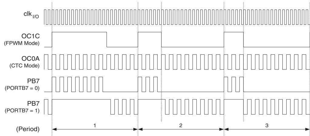
Figure 19-3. Output Compare Modulator, Timing Diagram
