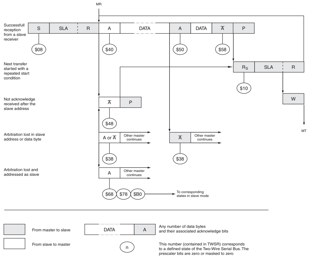
Figure 24-13. Formats and States in the Master Receiver Mode
