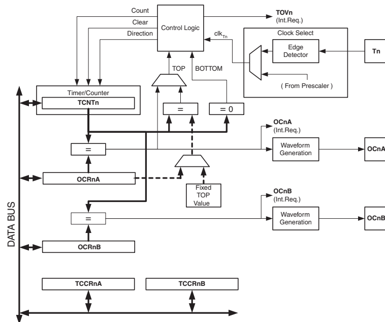
Figure 16-1. 8-bit Timer/Counter Block Diagram
