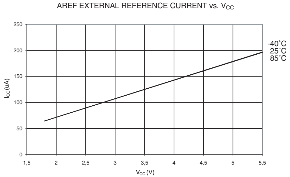
Figure 32-42. AREF External Reference Current vs. V_{CC}
