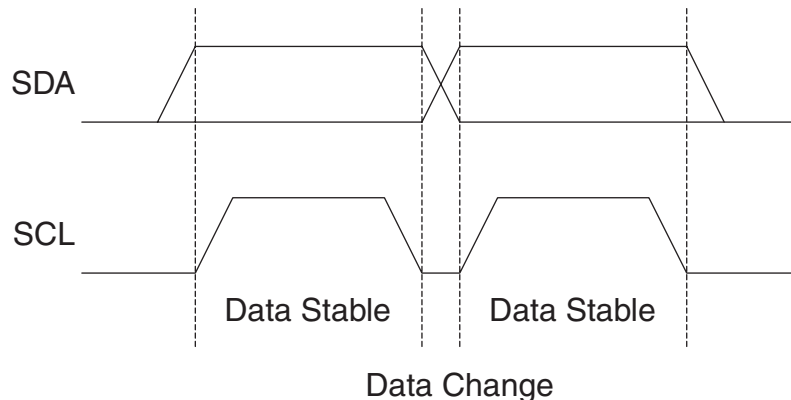
Figure 24-1. Data Validity
