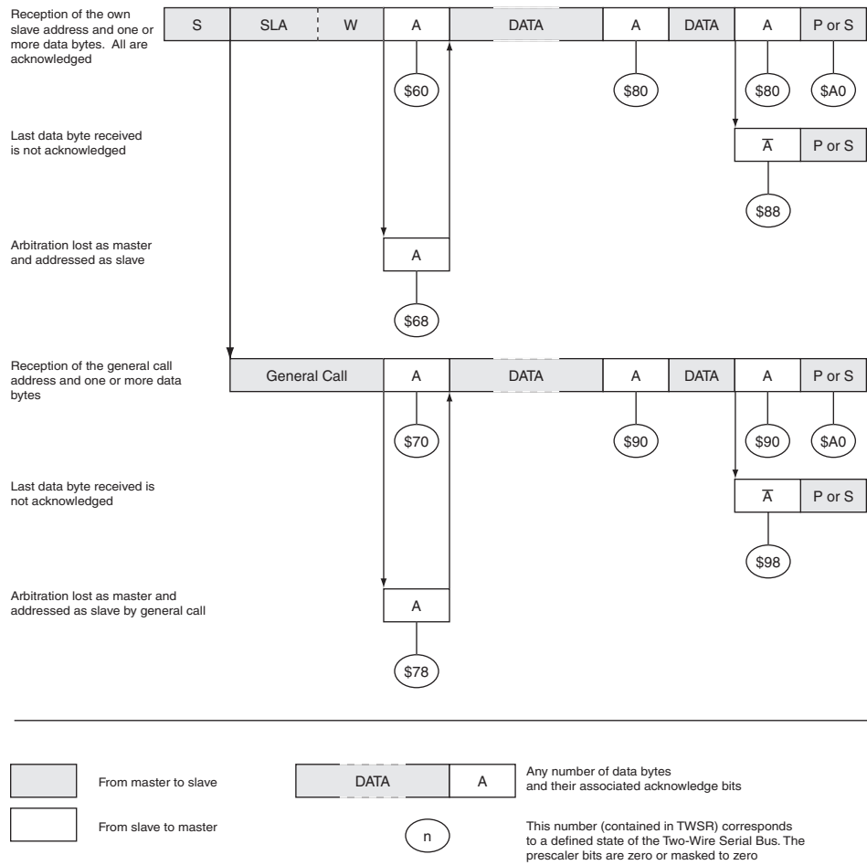
Figure 24-15. Formats and States in the Slave Receiver Mode
