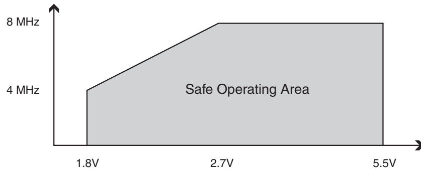
Figure 31-2. Maximum Frequency vs. V_{CC} when only using No-Read-While-Write Section (1) , ATmega2560V/ATmega2561V
