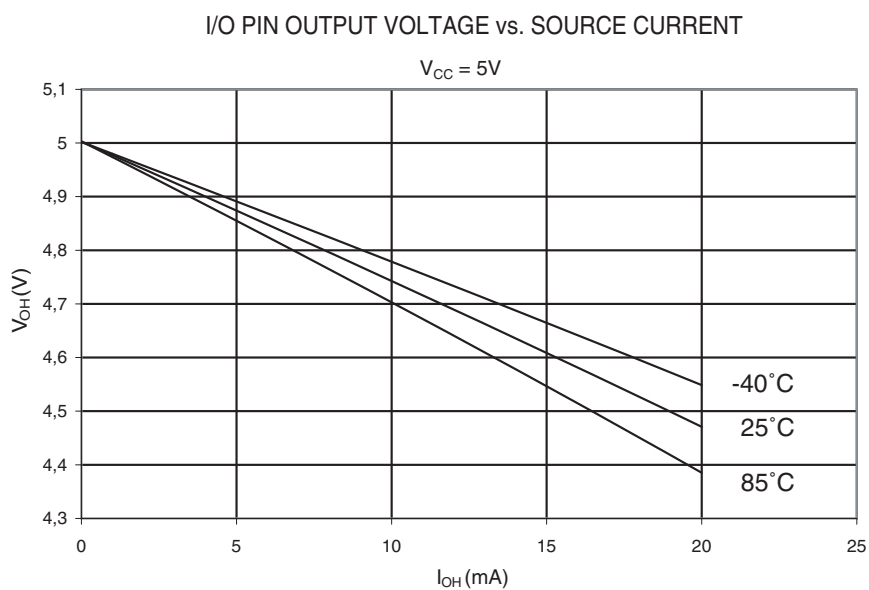
Figure 32-25. I/O Pin Output Voltage vs. Source Current ( V_{CC} = 5\text{ V} )
