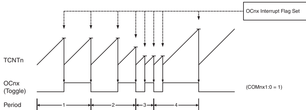
Figure 20-3. CTC Mode, Timing Diagram
