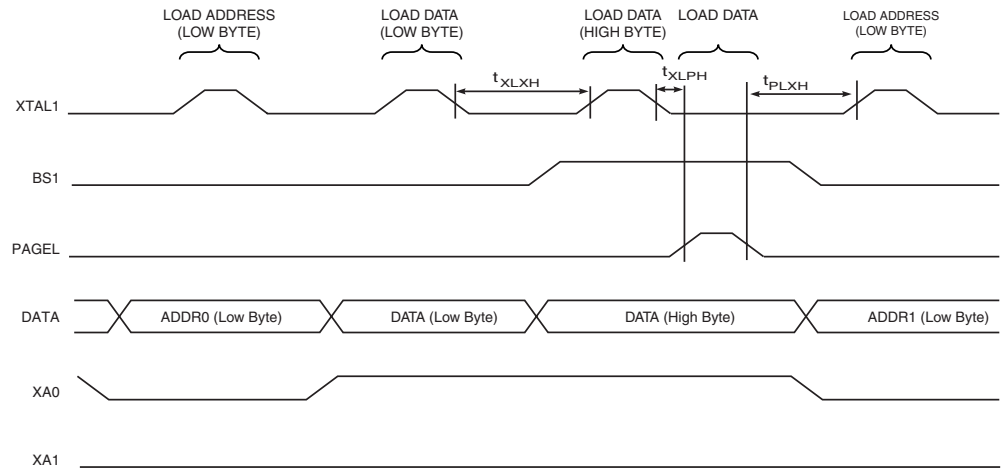
Figure 30-7. Parallel Programming Timing, Loading Sequence with Timing Requirements (Note:)
