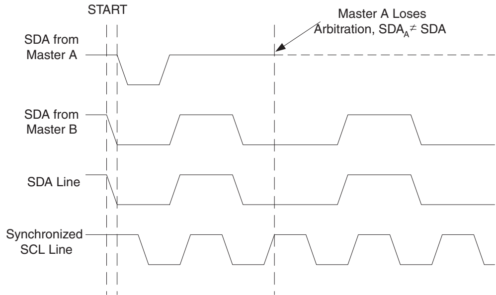
Figure 24-7. Arbitration Between Two Masters
