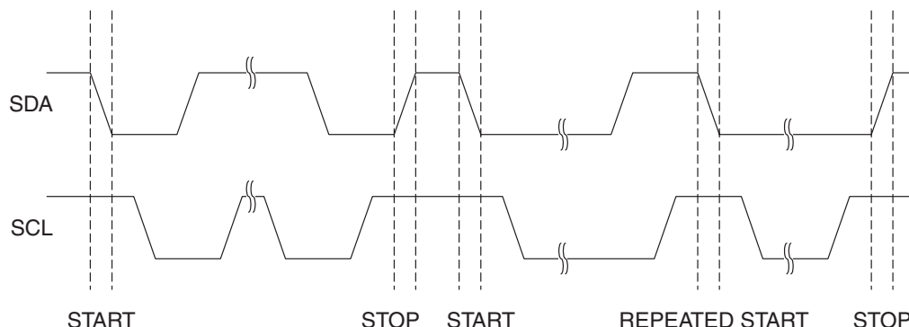
Figure 24-2. START, REPEATED START and STOP conditions
