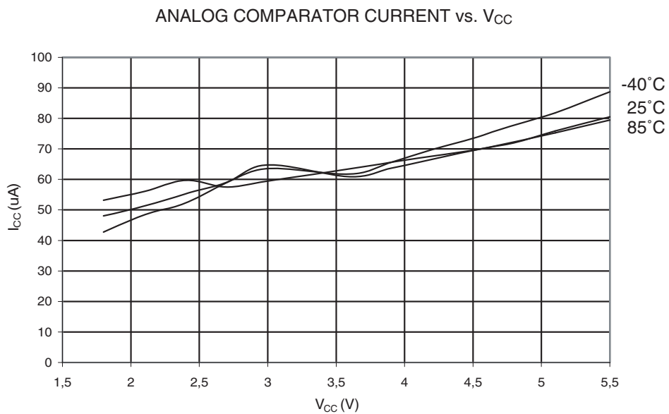
Figure 32-44. Analog Comparator Current vs. V_{CC}
