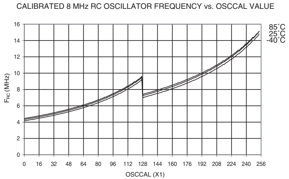
Figure 32-39. Calibrated 8 MHz RC Oscillator Frequency vs. Oscal Value
