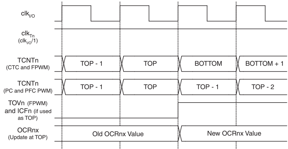
Figure 17-11. Timer/Counter Timing Diagram, no Prescaling
