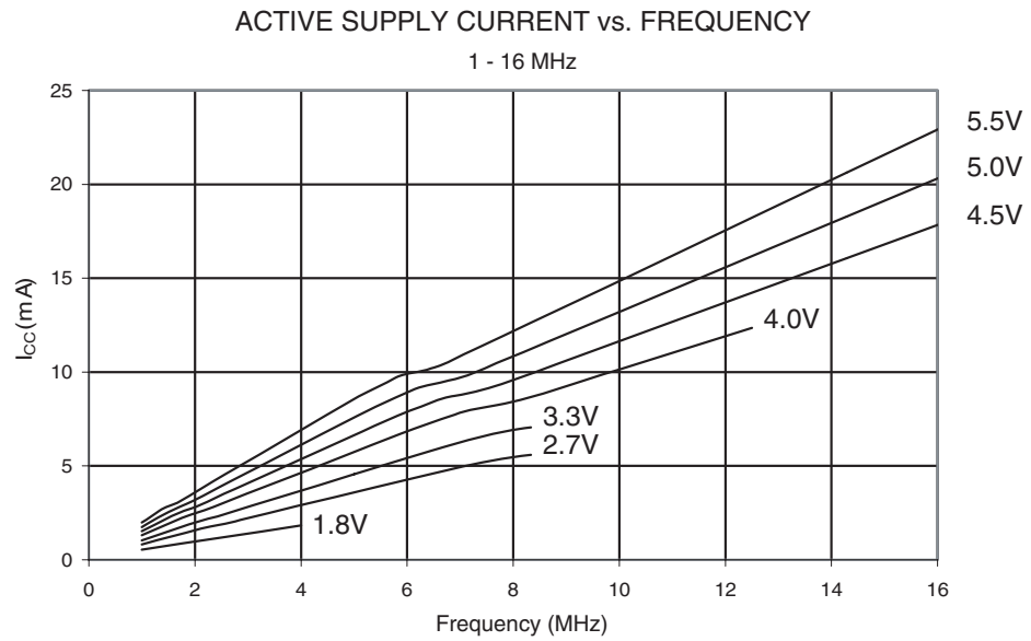
Figure 32-2. Active Supply Current vs. Frequency (1 - 16 MHz)
