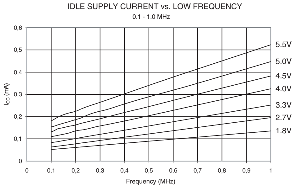
Figure 32-6. Idle Supply Current vs. Low Frequency (0.1 - 1.0 MHz)
