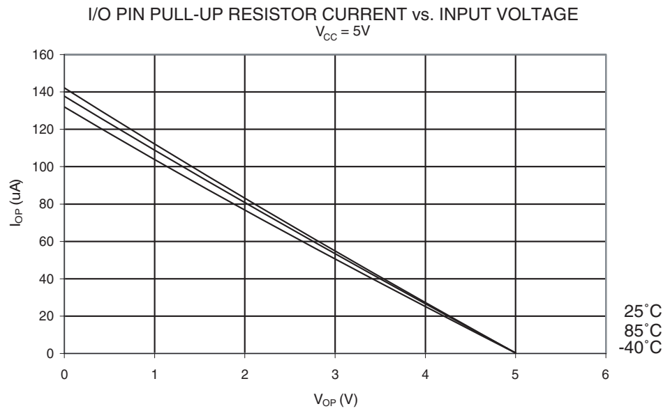
Figure 32-18. I/O Pin Pull-up Resistor Current vs. Input Voltage ( V_{CC} = 5V )
