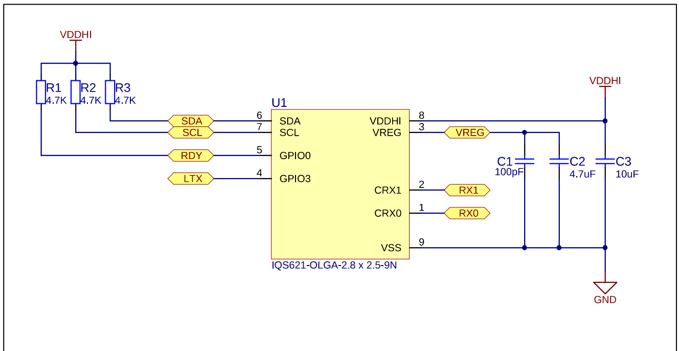
Figure 1.3 IQS621 reference schematic
