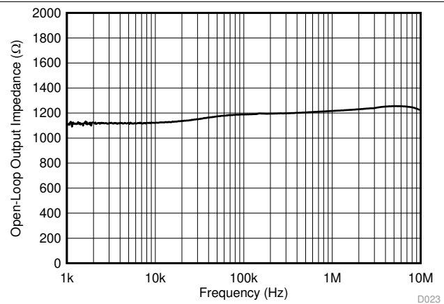
Figure 20. Open-Loop Output Impedance vs Frequency
