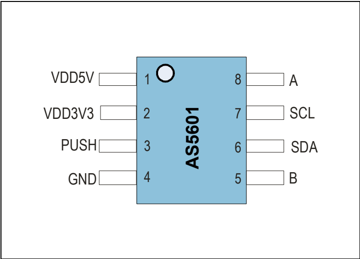
Figure 3: SOIC-8 Pin-Out
