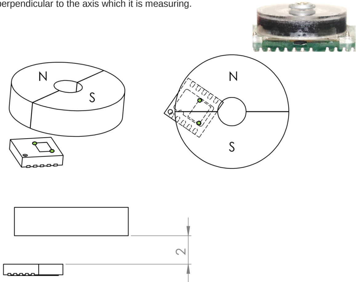
Figure 12-3 Magnet's position relative to IC with on-axis orientation Typical specifications of on-axis magnet position
