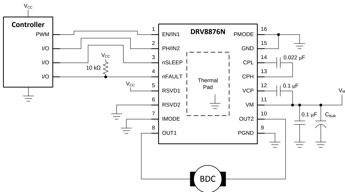
Figure 12. Typical Application Schematic
