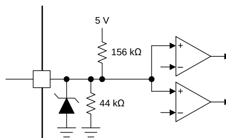
Figure 10. PMODE Tri-Level Input
