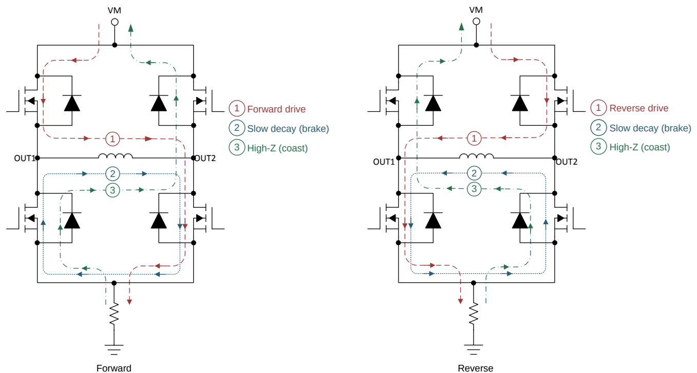
Figure 8. H-Bridge States
