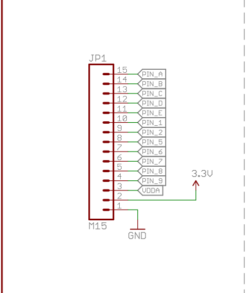
Pin Breakout
