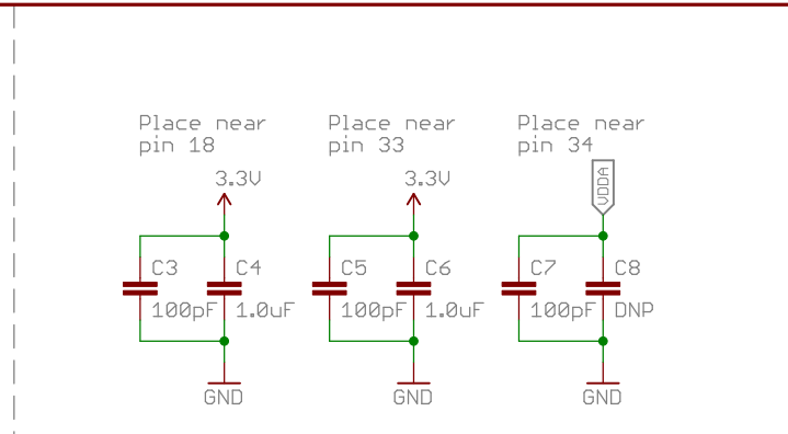
Decoupling Capacitors
