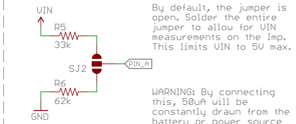
Input Voltage Measurement
