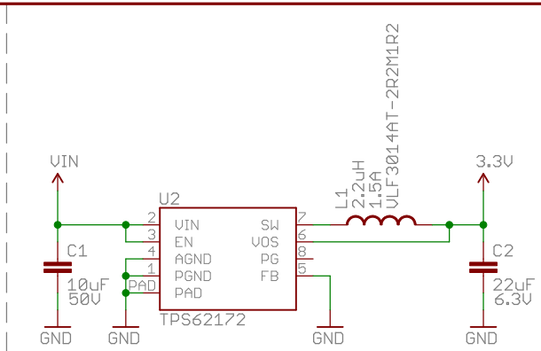
DC/DC Converter
